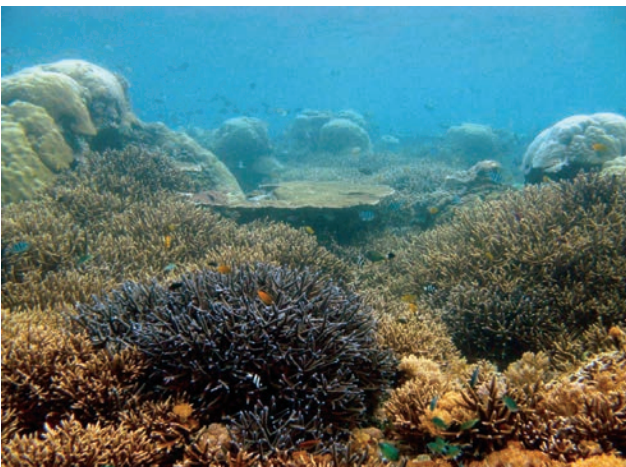
Plate 5.3. High cover of reef-building corals, Nusa Penida Station N4.2, composed predominantly by Acropora spp. and Porites spp.
