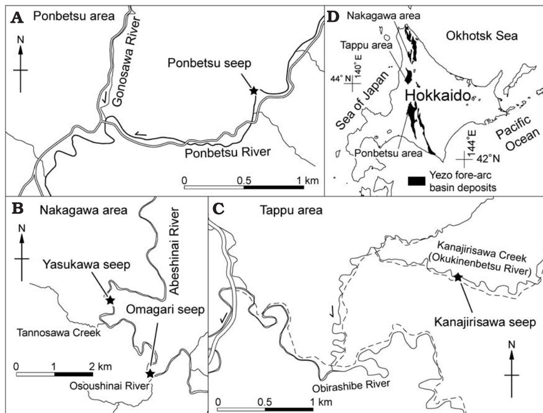
Fig. 1. Maps showing the fossiliferous seep deposits. A. The Albian Ponbetsu site. B. The Campanian Yasukawa and Omagari sites. C. The Cenomanian Kanajirisawa site. D. Overview.
