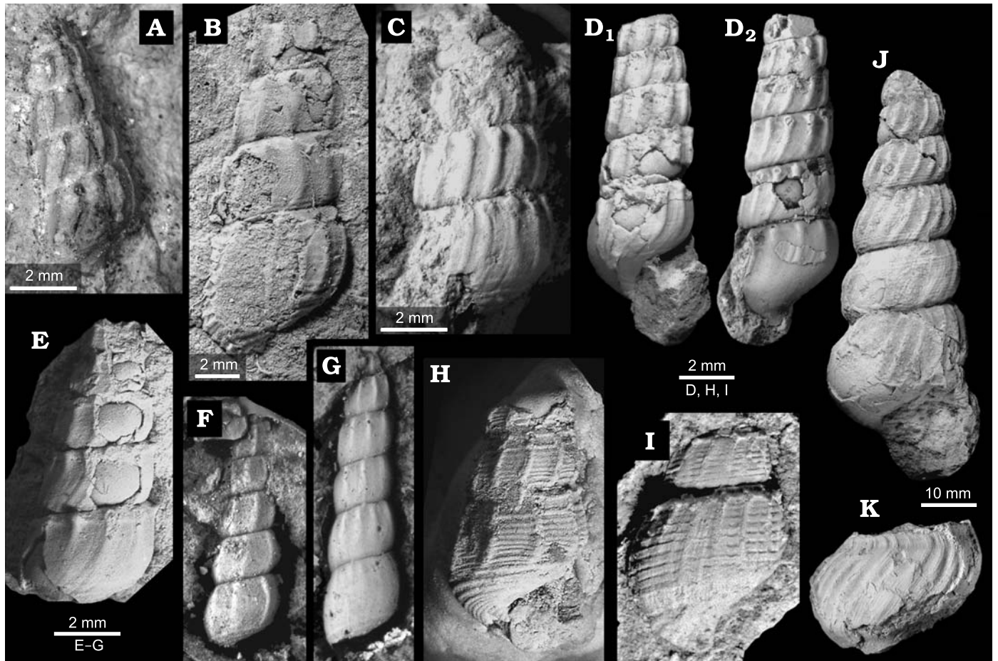
Fig. 5. Late Jurassic and Early Cretaceous abyssochrysois Hokkaidoconcha spp. and Abyssochrysis? giganteum sp. nov. from seep carbonates in California, USA. A–C. Hokkaidoconcha occidentalis (Stanton, 1895). A. Lectotype (USNM 23077) from Paskenta (Tithonian; site 2). B. Specimen (CAS 70391) with well-developed spiral sculpture from Wilbur Springs (Hauterivian; site 5). C. Specimen (UCMP 555091) with poorly developed spiral sculpture from NW Berryessa (Tithonian; site 10). D, E. Hokkaidoconcha tehamaensis sp. nov. from Paskenta (Tithonian; site 10). D. Holotype (UCMP 555092); apertural ( D 1 ) and lateral ( D 2 ) views. E. Paratype (CAS 70390), note fading axial ribs on flank. F, G. Hokkaidoconcha morenoensis sp. nov. from Moreno Gulch (Santonian; site 14) F. Holotype (LACMIP 13483) with well-developed axial ribs and spiral sculpture on base. G. Paratype (LACMIP 13484) with fading axial ribs on later whorls. H. Hokkaidoconcha bilirata sp. nov., holotype (UCMP 555093) from Wilbur Springs (Hauterivian; site 5). I. Hokkaidoconcha sp. (UCMP 555094) from NW Berryessa (Tithonian; site 10). J, K. Abyssochrysis? giganteum sp. nov. from E Berryessa (Lower Cretaceous; site 12). J. Holotype (UCMP 555095). K. Paratype (UCMP 555096).
