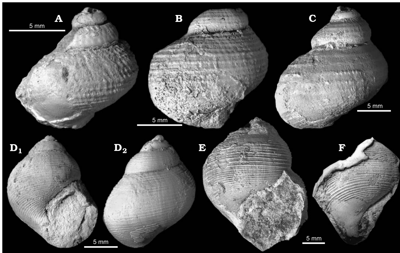
Fig. 7. Abyssochrysoid gastropod Paskentana spp. from Late Jurassic and Early Cretaceous seep carbonates in California, USA. A–C. Paskentana berryessaensis sp. nov. A. Holotype (UCMP 555098), small specimen with nodular sculpture from NW Berryessa (Tithonian; site 10). B. Paratype (UCMP 555099), specimen with beaded spiral cords from NW Berryessa (Tithonian; site 10). C. Paratype (UCMP 555100) from Bear Creek (Valanginian; site 4), specimen with spiral sculpture and fine axial growth increments. D–F. Paskentana globosa sp. nov. D. Paratype (UCMP 555101) from Little Indian Valley (Valanginian?; site 6). E. Holotype (CAS 70394), large specimen from Knoxville (Early Cretaceous?, site 9). F. Rubber cast of a last whorl, from Knoxville.
