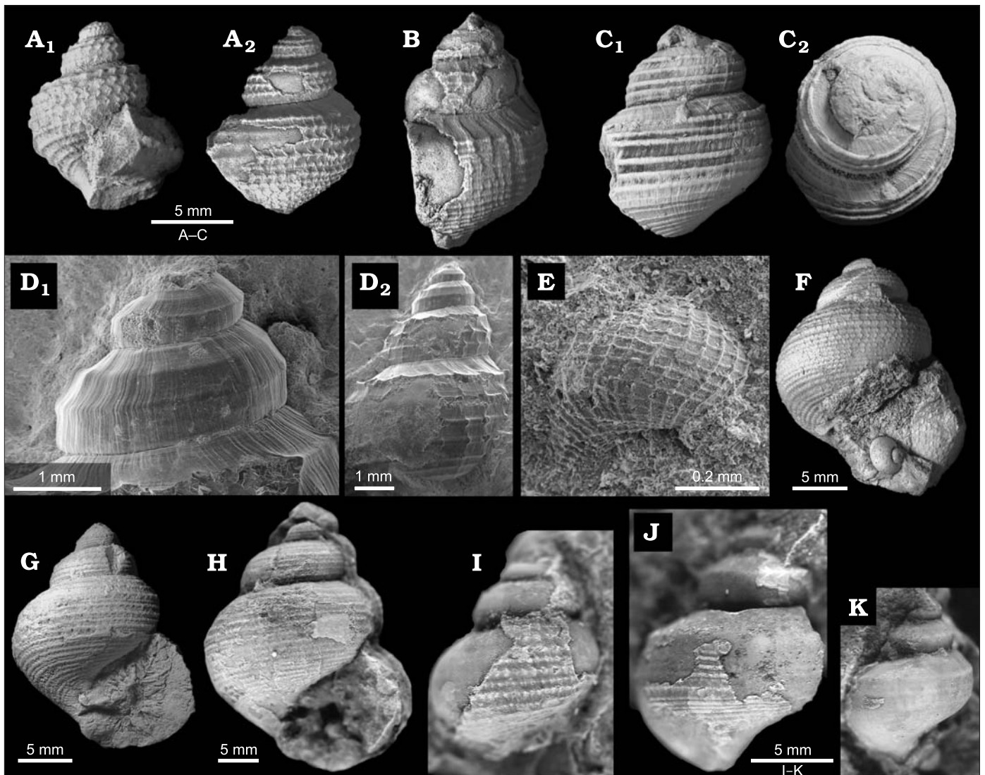
Fig. 6. Abyssochrysid gastropod Paskentana paskentaensis (Stanton, 1895) from Late Jurassic and Early Cretaceous seep carbonates in California, USA. A. Small specimen (CAS 70392) with strong scaly sculpature from Bear Creek (Valanginian; site 4); apertural ( A 1 ) and lateral ( A 2 ) views. B. Specimen (CAS 70393) with broad shoulder from Bear Creek (Valanginian; site 4). C. Specimen (UCMP 555097) with broad shoulder and almost smooth spiral sculpature, from Little Indian Valley (Valanginian?; site 6). D. Juvenile specimen (UCMP 555104) from Bear Creek (Valanginian; site 4), close-up on first whorls ( D 1 ) and entire specimen ( D 2 ). E. Isolated partial larval shell (UCMP 555105) from Bear Creek (Valanginian; site 4) that most likely belongs to Paskentana paskentaensis . F. Specimen (UCMP 154113) without shoulder and fine scaly sculpature, from Rice Valley (Hauterivian?; site 3). G. Specimen (UCMP 13701) without shoulder, from Wilbur Springs (Hauterivian; site 5). H. “ Turbo ” wilburensis Stanton, 1895 (pl. 12: 15), lectotype (USNM 23068) from Wilbur Springs (Hauterivian; site 5). I. “ Turbo ” paskentaensis Stanton, 1895 (pl. 12: 6), lectotype (USNM 23067) from Paskenta (Tithonian; site 2). J, K. “ Turbo ” humerosus Stanton, 1895 from Wilbur Springs (Hauterivian; site 5). J. Lectotype (USNM 23072). K. Paralectotype (specimen illustrated by Stanton 1895: pl. 12: 10).
