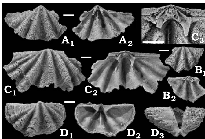
Fig. 33. Spiriferelline brachiopod Spiriferellina cf. insculpta (Phillips, 1836) from the Tournaisian Muhua Formation, southern China. A. Ventral valve, PKUM02-0578, in exterior (A 1 ) and interior (A 2 ) views. B, C. Two incomplete dorsal valves, PKUM02-0579 (B) and PKUM02-0388 (C, same as in Fig. 7B), in exterior (B 1 , C 1 ) and interior (B 2 , C 2 ) views, and enlargement of cardinalia (C 3 ). D. Ventral valve, PKUM02-0580, in exterior (D 1 ), interior (D 2 ), and posterior (D 3 ) views. Sample MH2 (A, B, D) and GB (C). Scale bars 2 mm.
