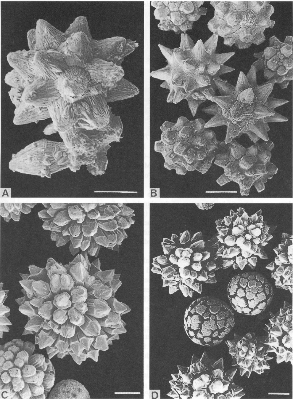
Figure 7. Spicules: A, Didemnum nocturnum ; B, Polysyncraton millepore ; C, D, Polysyncraton rostrum . Scale bars = 10 \mu m.
