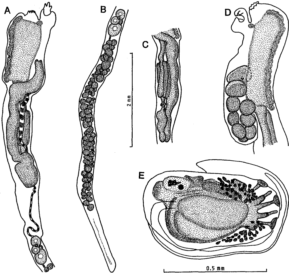
Figure 9. Aplidium colini sp. nov.: A, B, zoid; C, abdomen; D, brooded embryos; E, larva.
