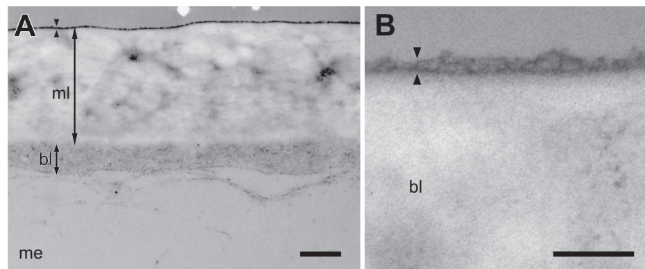
Fig. 1. Exumbrellar surface of Colobonema sericeum . (A) The exumbrellar surface of the mesoglea is covered with a three-layered sheet, which includes the outer, middle (ml), and basal layers (bl). (B) Enlargement of the outer layer overlying the middle layer. Facing arrowheads indicate the outer layer. bl, basal layer; me, mesoglea; ml, middle layer. Scale bars: 0.5 \mu m for (A) , 0.2 \mu m for (B) .
