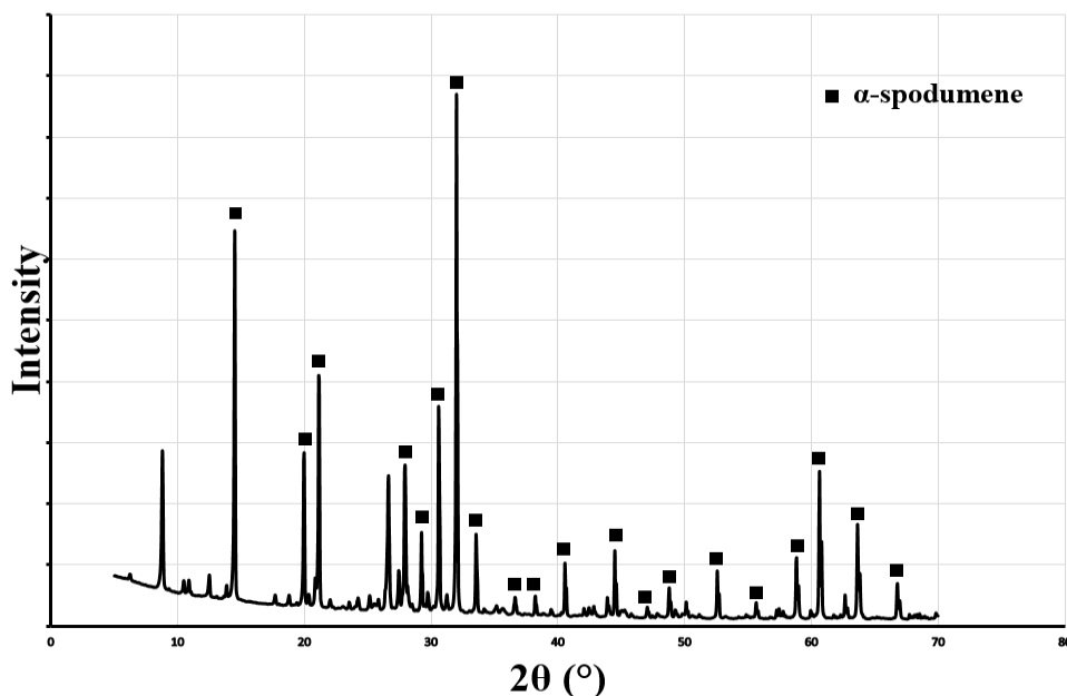
Figure 6. X-Ray pattern of a typical \alpha -spodumene sample, only the main peaks of \alpha -spodumene are indicated.
