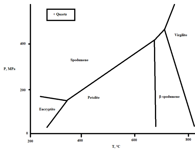
Figure 4. Stability relations among eucryptite ( \text{LiAlSiO}_4 ), \alpha -spodumene ( \text{LiAlSi}_2\text{O}_6 ), petalite ( \text{LiAlSi}_4\text{O}_{10} ), \beta -spodumene ( \text{LiAlSi}_5\text{O}_{12} ) and virgilite ( \text{LiAlSi}_5\text{O}_{12} ), in the system \text{LiAlSiO}_4\text{-SiO}_2\text{-H}_2\text{O} [30] (adapted with permission from the Mineralogical Society of America, American Mineralogist; published by the Mineralogical Society of America, 2019).
