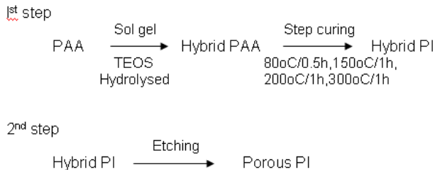
Scheme 4. Preparation of porous Polyimide using sol-gel method
