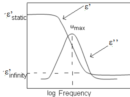
Figure 5. Debye dielectric dispersion curve.
