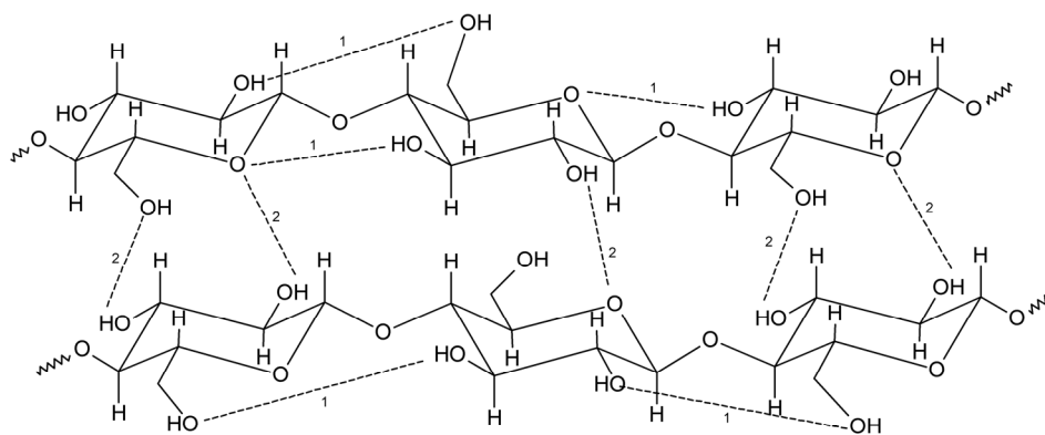
Figure 1. The structure and intra- (1) and interchain (2) hydrogen bonding pattern in cellulose.
