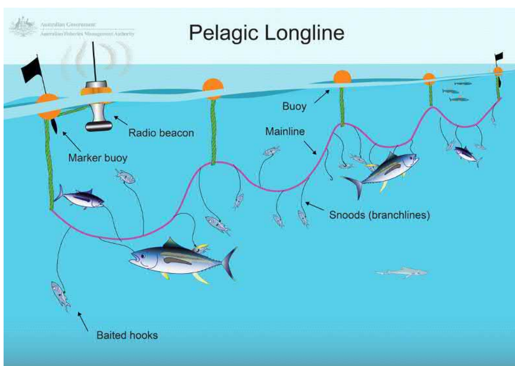
FIGURE 7-32: TYPICAL PELAGIC LONGLINE GEAR CONFIGURATION
