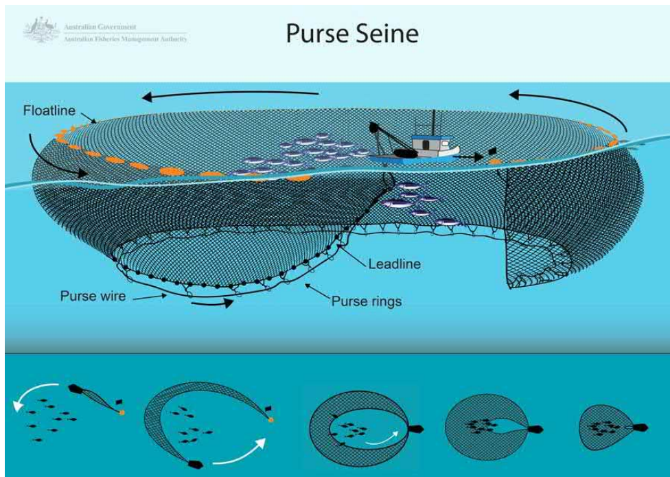
FIGURE 7-29: SCHEMATIC OF TYPICAL PURSE-SEINE GEAR DEPLOYED IN THE “SMALL” PELAGIC FISHERY
