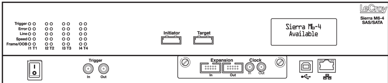
Figure 1.2: Front Panel
