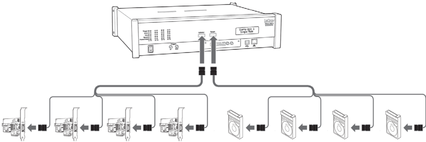
Figure 1.7: Sierra M6-4 Single Lane Connections
