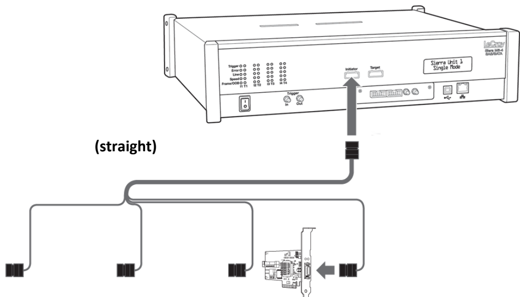
Figure 1.6: Sierra M6-4 Device Emulator Connected to DUT
