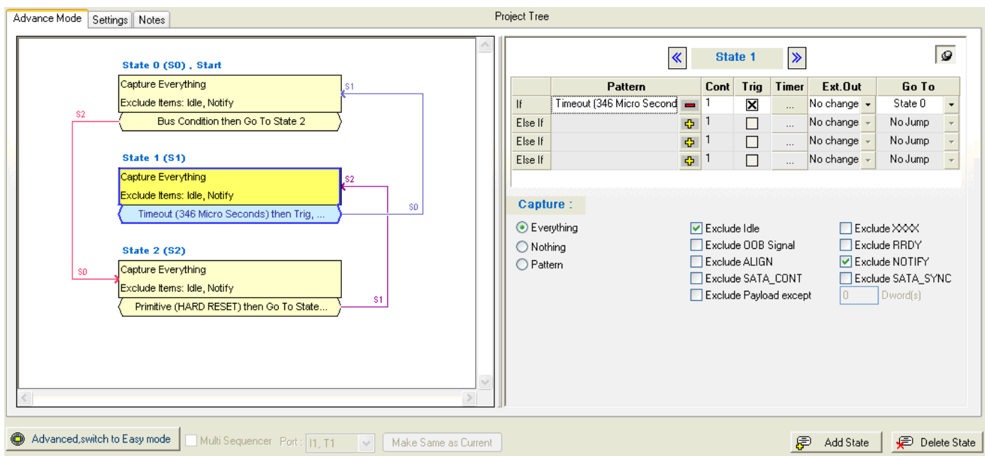
Figure 2.85: State Machine with Timeout Pattern to Replace Timer
