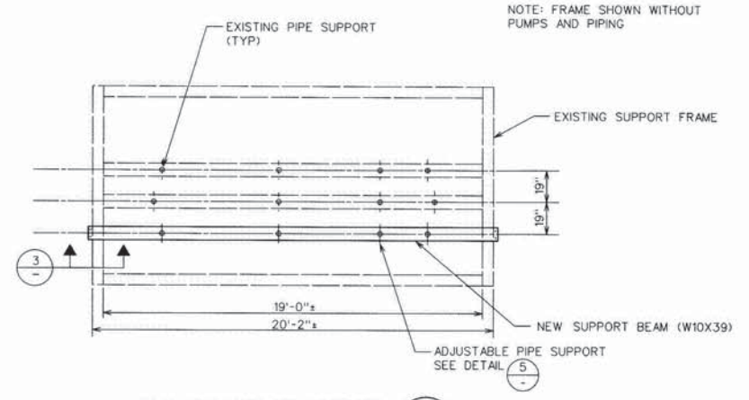
PUMP FRAME SUPPORT 2 SCALE: 1"=4'-0"
