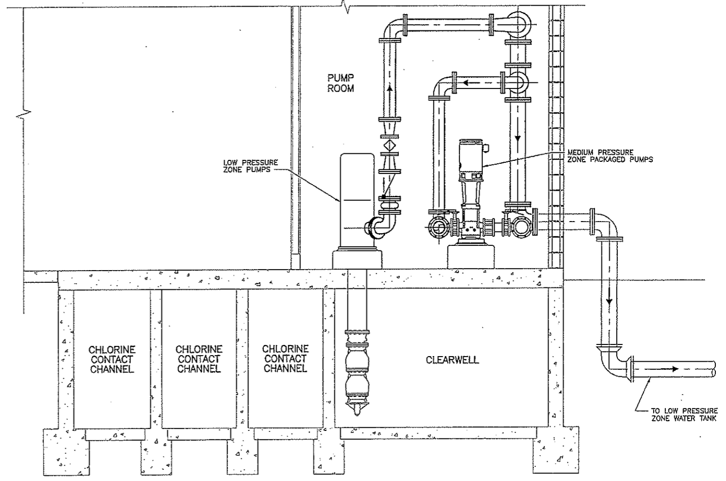
SECTION B 1/4" = 1'-0"
