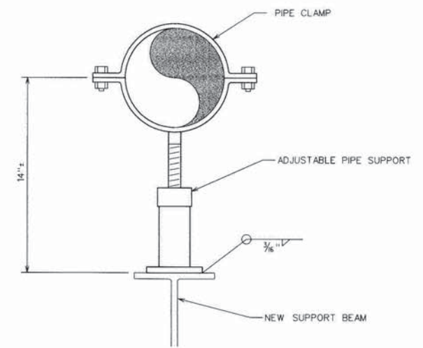
ADJUSTABLE PIPE SUPPORT 5 NO SCALE
