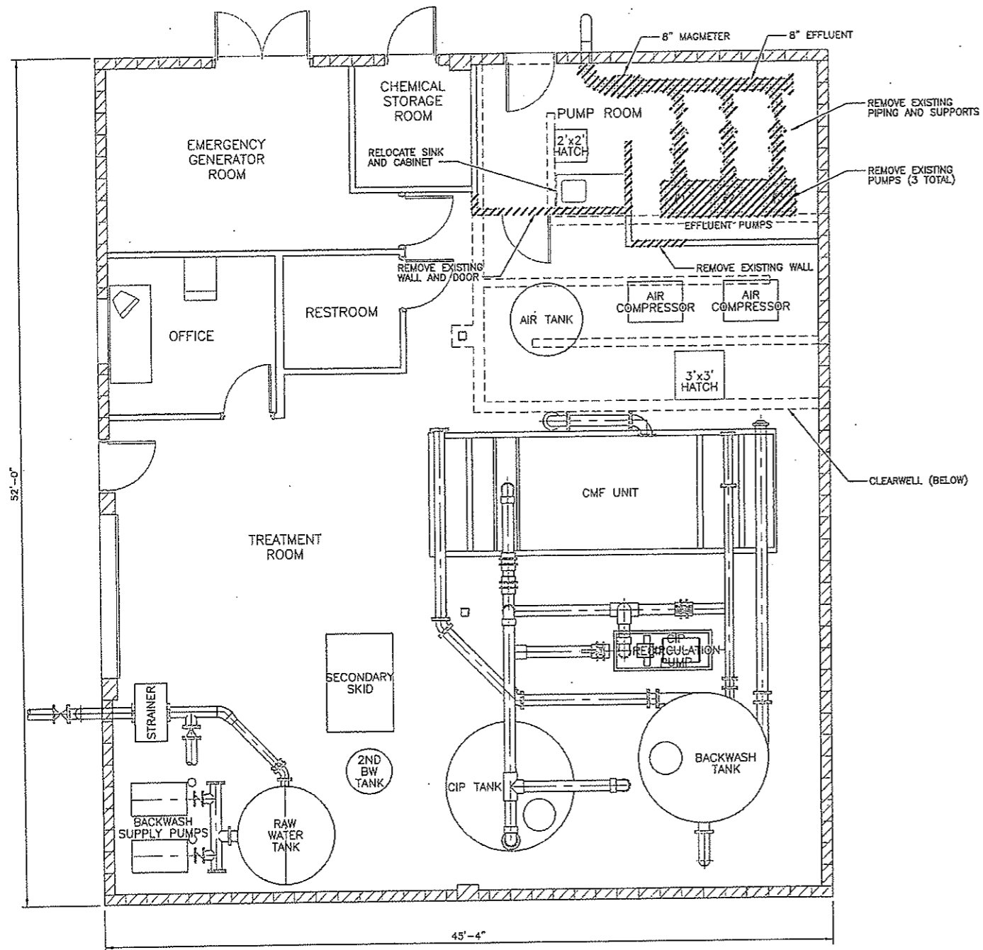
FLOOR PLAN MODIFICATIONS 1/8" = 1'-0"
