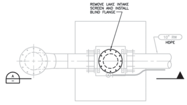
EXISTING LAKE INTAKE MODIFICATION PLAN 3/4" = 1'-0" 2 SHT 2
