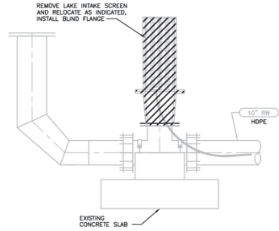
EXISTING LAKE INTAKE MODIFICATION SECTION 3/4" = 1'-0" A
