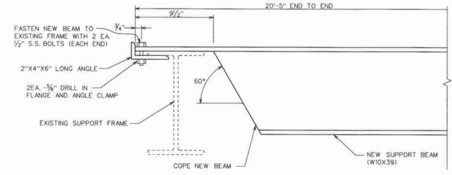
CONNECTION 3 NO SCALE
