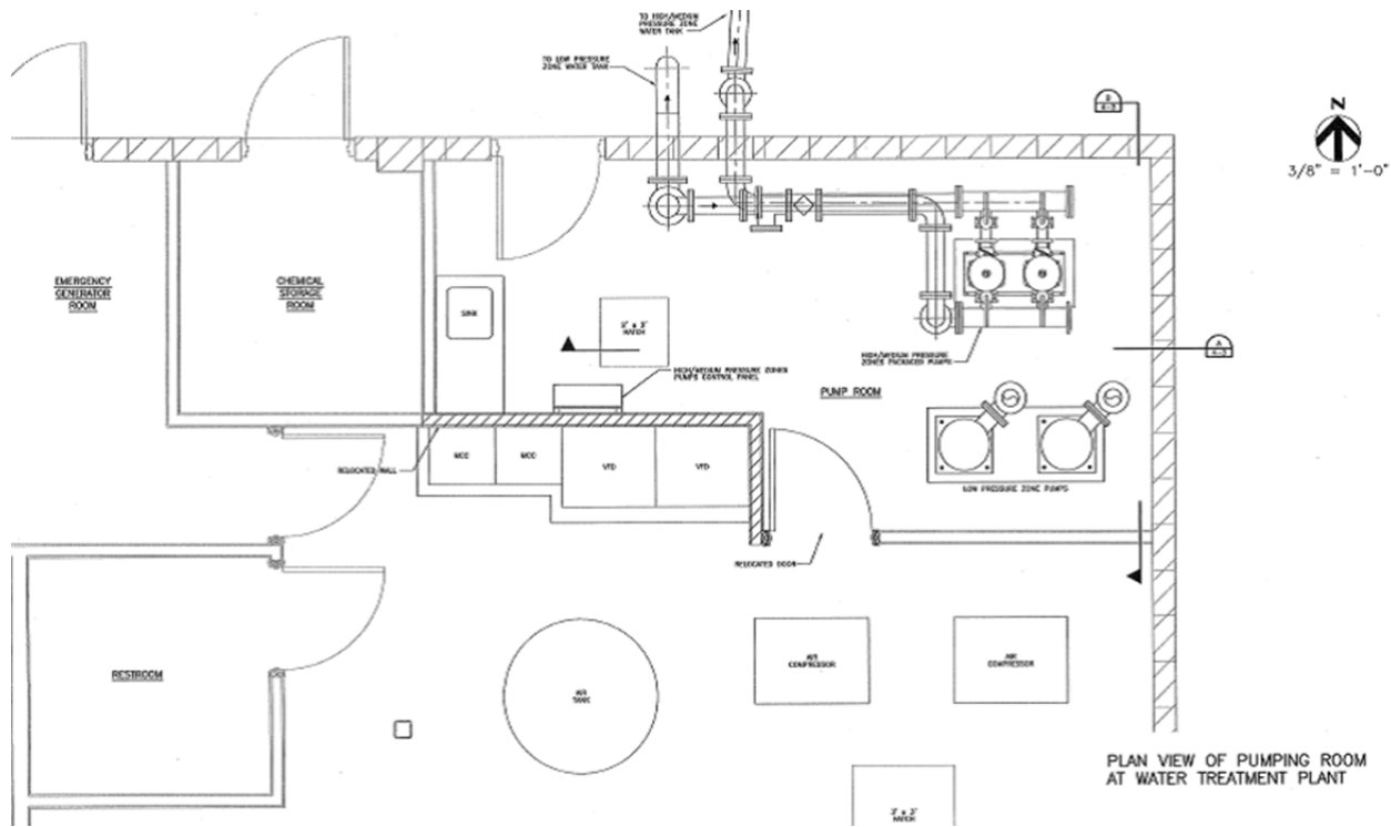
Figure 5-12 Alt 2 WTP Plan Pumping Modifications
