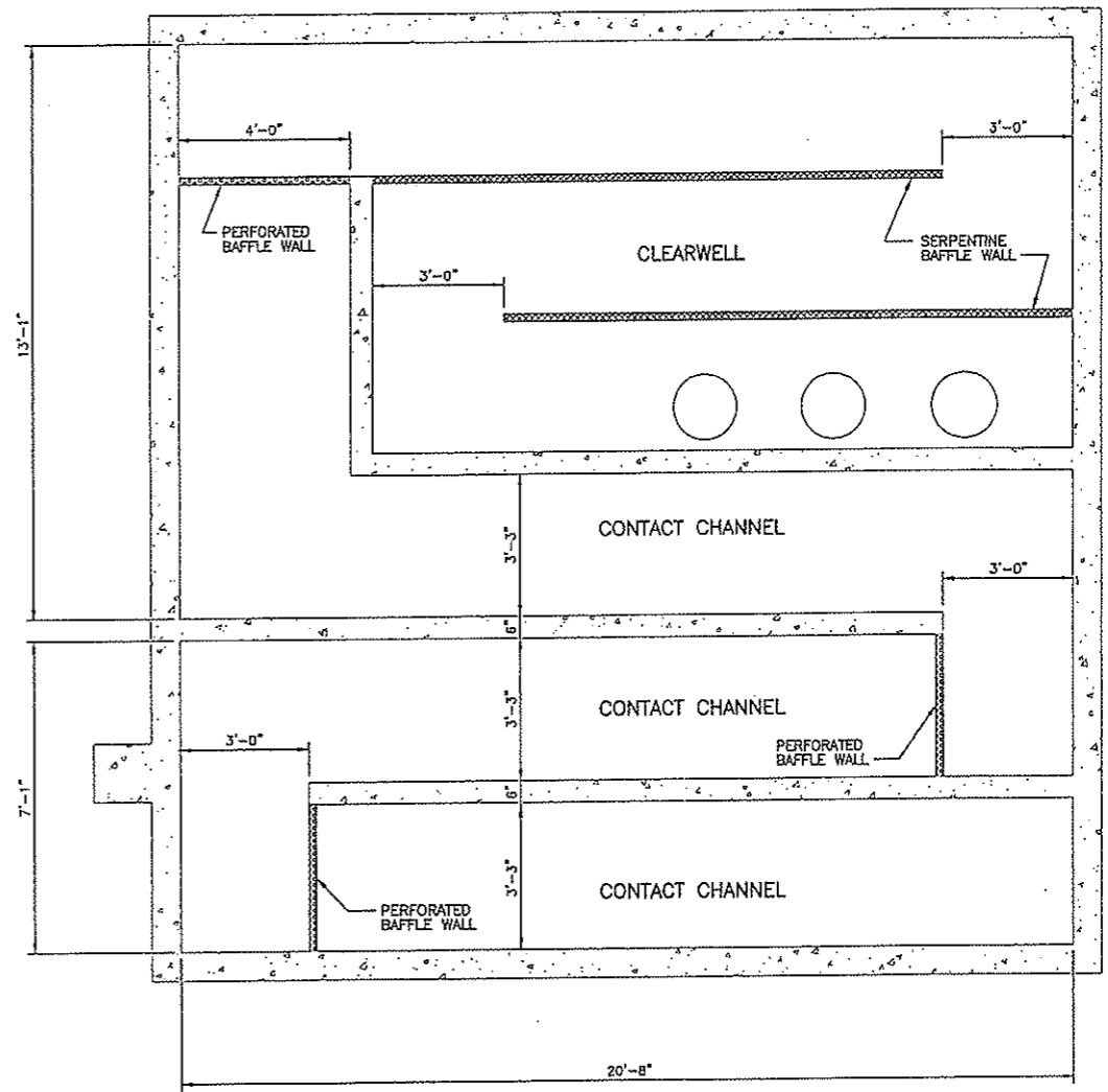
CLEARWELL: PLAN MODIFICATIONS 1/4" = 1'-0"
