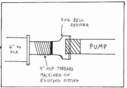
FITTINGS FOR 2 ORIGINAL PUMP CANS
