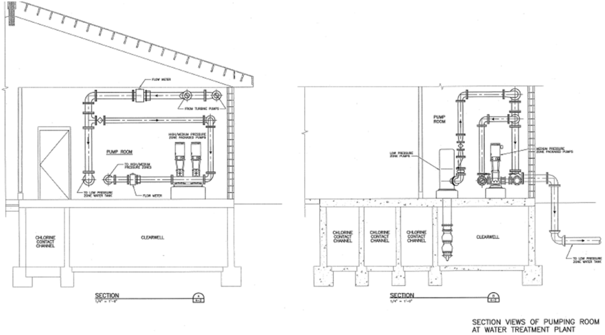
Figure 5-13 Alt 2 WTP Section Pumping Modifications
