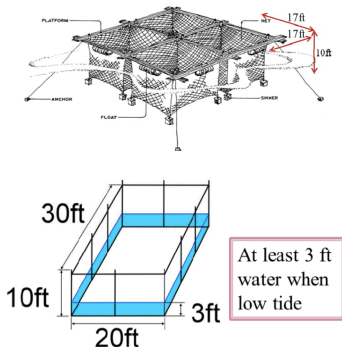
FIGURE 8. FLOATING FISH CAGE (ABOVE) AND FISH PEN (BELOW).
