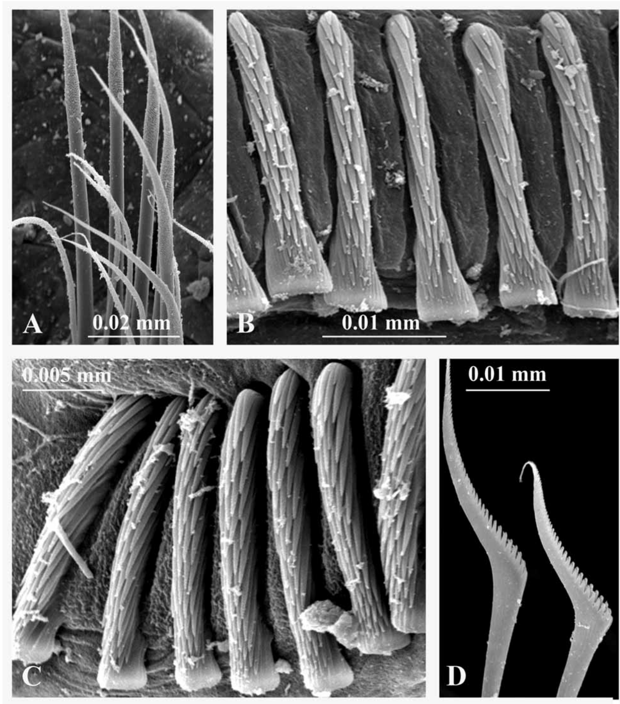
FIGURE 27. SEM micrographs of chaetae in Marifugia cavatica . Bosnia & Herzegovina, Ravno, Zavala, Vjetrenica, Ravanjski kanal, legit M. Zagmajster, det. E. Kupriyanova, SAM E3612. A—thoracic chaetae, B—thoracic uncini, C—anterior abdominal uncini, D—anterior abdominal chaetae with hollow tips.
