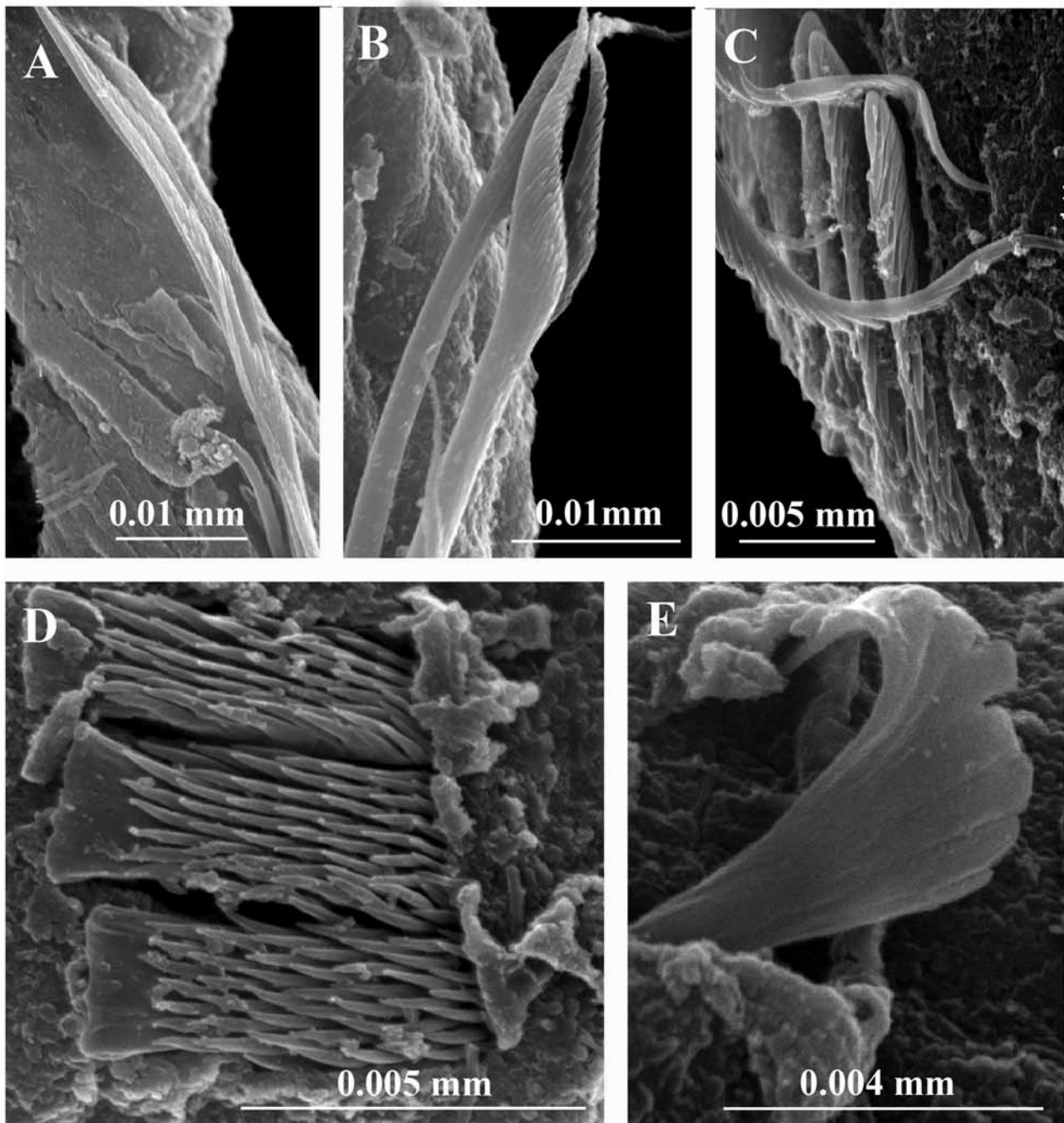
FIGURE 48. SEM micrographs of chaetae in Tanturia zibrowii . Israel, Gulf of Aqaba (Elat), Sinai coast, infauna of Dendropoma , paratype, exchange with HUI, ZMA V.Pol. 4668. A—fin-and-blade collar chaetae, B—thoracic chaetae, C—thoracic uncini, D—abdominal uncini, E—abdominal chaeta.
