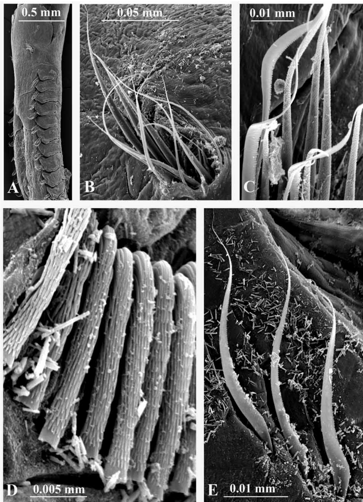
FIGURE 18. SEM micrographs of Filogranella elatensis . Israel, Elat, 10 m, legit J. Dafni, det. H.A. ten Hove, ex HUJ, SAM E3661. A—Lateral view of thorax, B—bundle of collar chaetae, C—thoracic chaetae of 4 th chaetiger ( Apomatus and "limbate"), D—anterior abdominal uncini, E—anterior abdominal chaetae.
