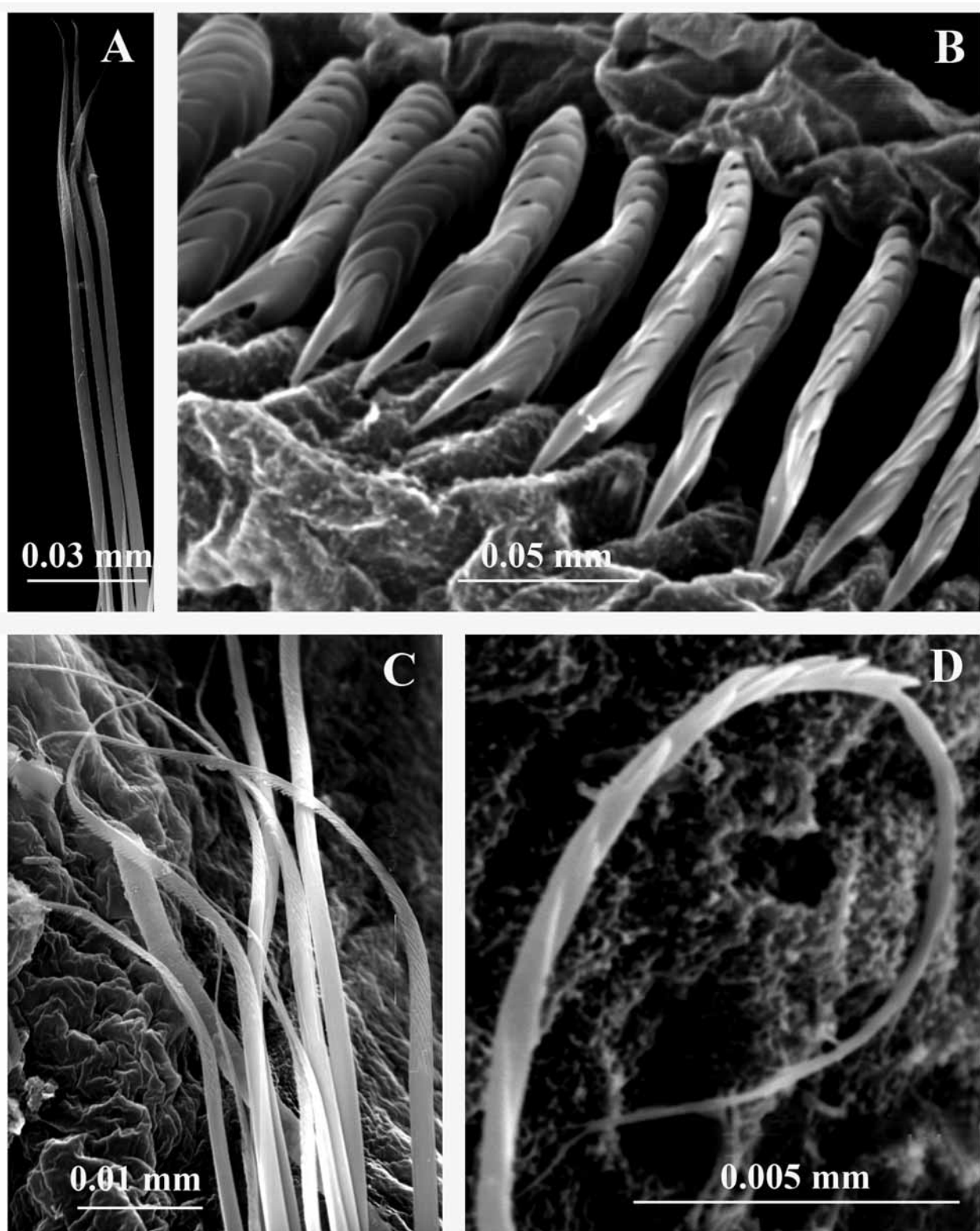
FIGURE 32. SEM micrographs of chaetae in Paraprotis dendrova . Australia, Queensland, Lizard Island, Granite Head, from underside of boulders on rock, little sand, subtidally, legit H.A. ten Hove, 18.06.1983, det. D. Makhan. A—bundle of collar chaetae, B—thoracic uncini, C—thoracic chaetae, D—abdominal chaeta.
