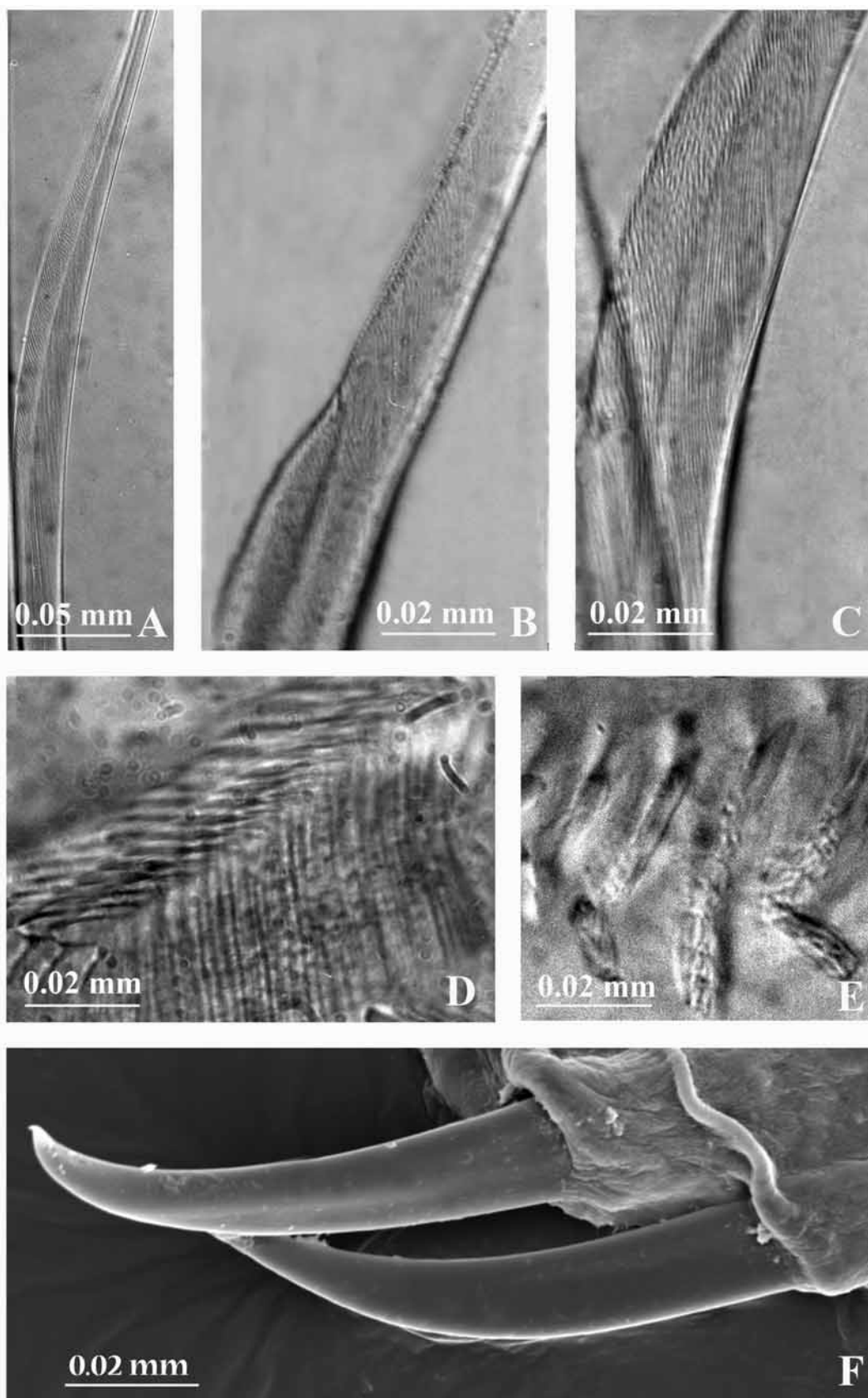
FIGURE 33. Photos (A–E) and a SEM micrograph (F) of chaetae in Paumotella takemoana . Holotype, USNM and MCZ (slides). A—“limbate” chaeta of 6 th thoracic chaetiger, B— Apomatus chaeta of 6 th chaetiger, C—same Apomatus chaeta as in B, but different focus, D—lateral view of thoracic uncini, E—frontal view of abdominal uncini, F—acicular abdominal chaetae.
