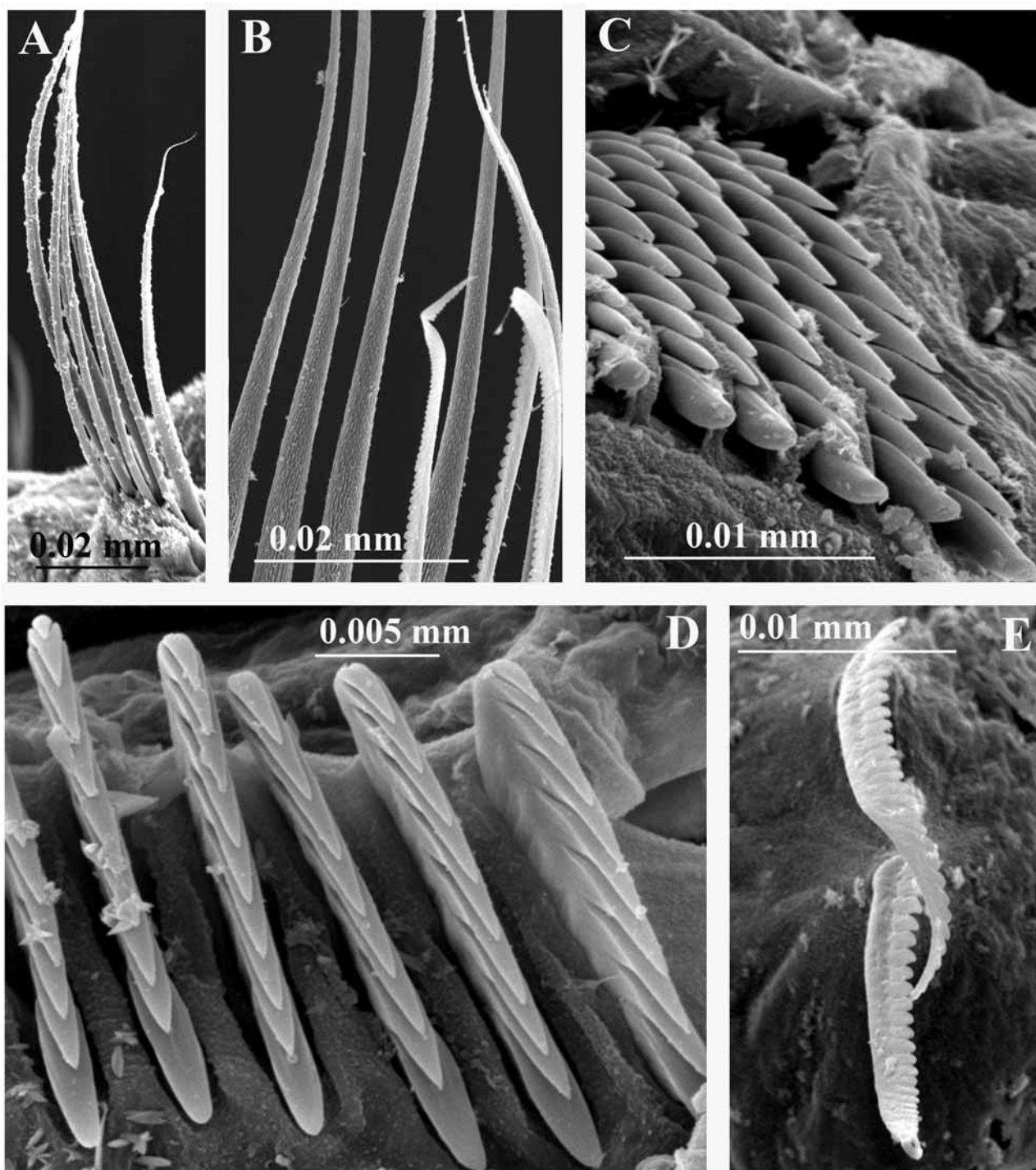
FIGURE 28. SEM micrographs of chaetae in Metavermilia acanthophora . Australia, Queensland, Lizard Island, legit G. Rouse and E. Kupriyanova, det. E. Kupriyanova. A—bundle of collar chaetae, B—thoracic “limbate” and Apomatus chaetae, C—thoracic uncini, D—anterior abdominal uncini, E—anterior abdominal chaetae.
