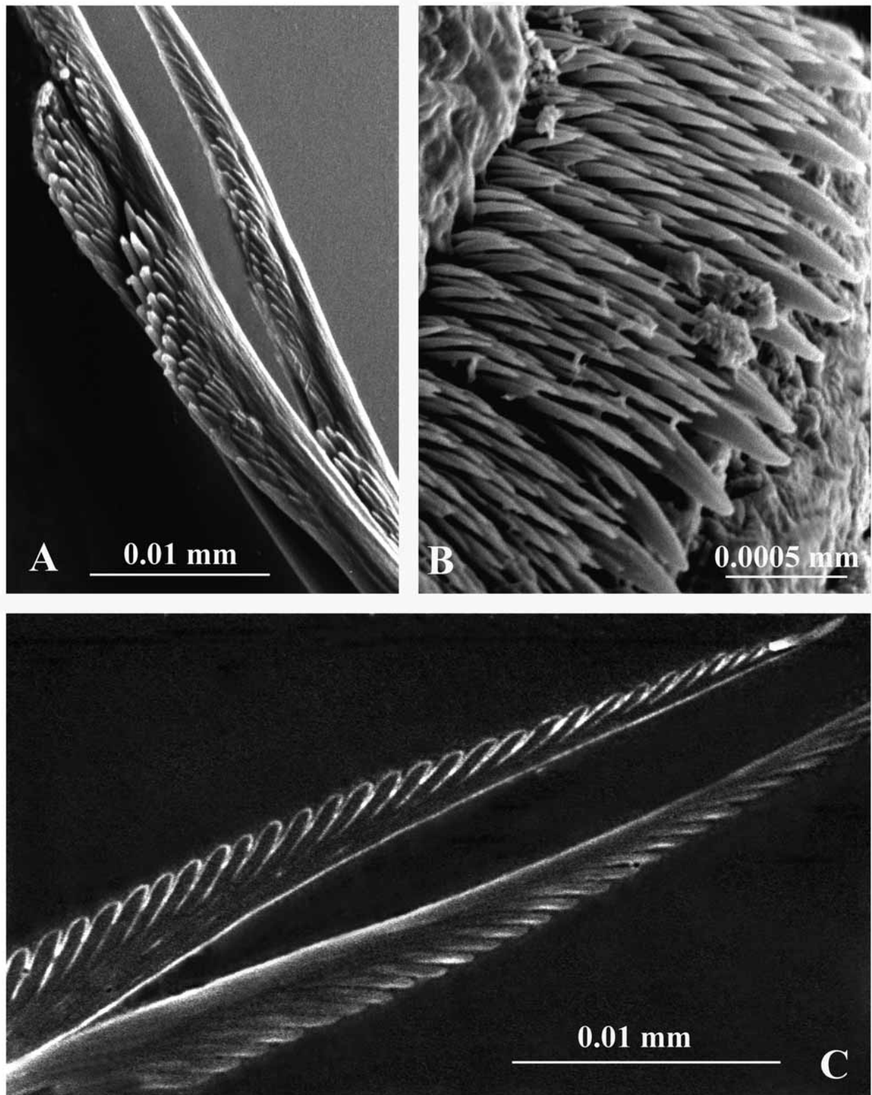
FIGURE 17. SEM micrographs of chaetae in Filograna implexa . United Kingdom, Orkney Islands, Head of Work, 22 m, legit M.J. de Kluyver, ZMA V.Pol. 3767. A—fin-and-blade collar chaetae, B—1 st row of thoracic uncini, C—middle abdominal chaetae, imprint of tip.
