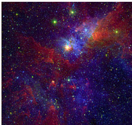
Great nebula in Carina, surrounding Eta Carinae
