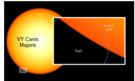
Size comparison between the diameter of the Sun and VY Canis Majoris, a hypergiant which is among the largest known stars
