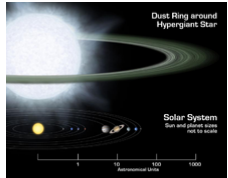
A hypergiant star and its protoplanetary disk compared to the size of the Solar System
