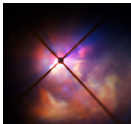
Very Large Telescope image of the surroundings of VY Canis Majoris
