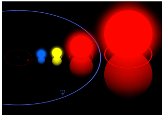
Comparison of the Pistol Star, Rho Cassiopeiae, Betelgeuse, and VY Canis Majoris superimposed on an outline of the Solar System. The blue half-ring centered near the left edge represents the orbit of Neptune, the outermost planet of the Solar System.
