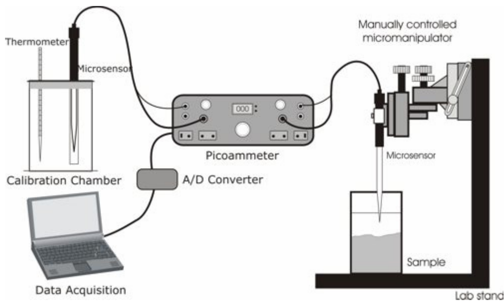
Figure 3. Microelectrode set-up.
