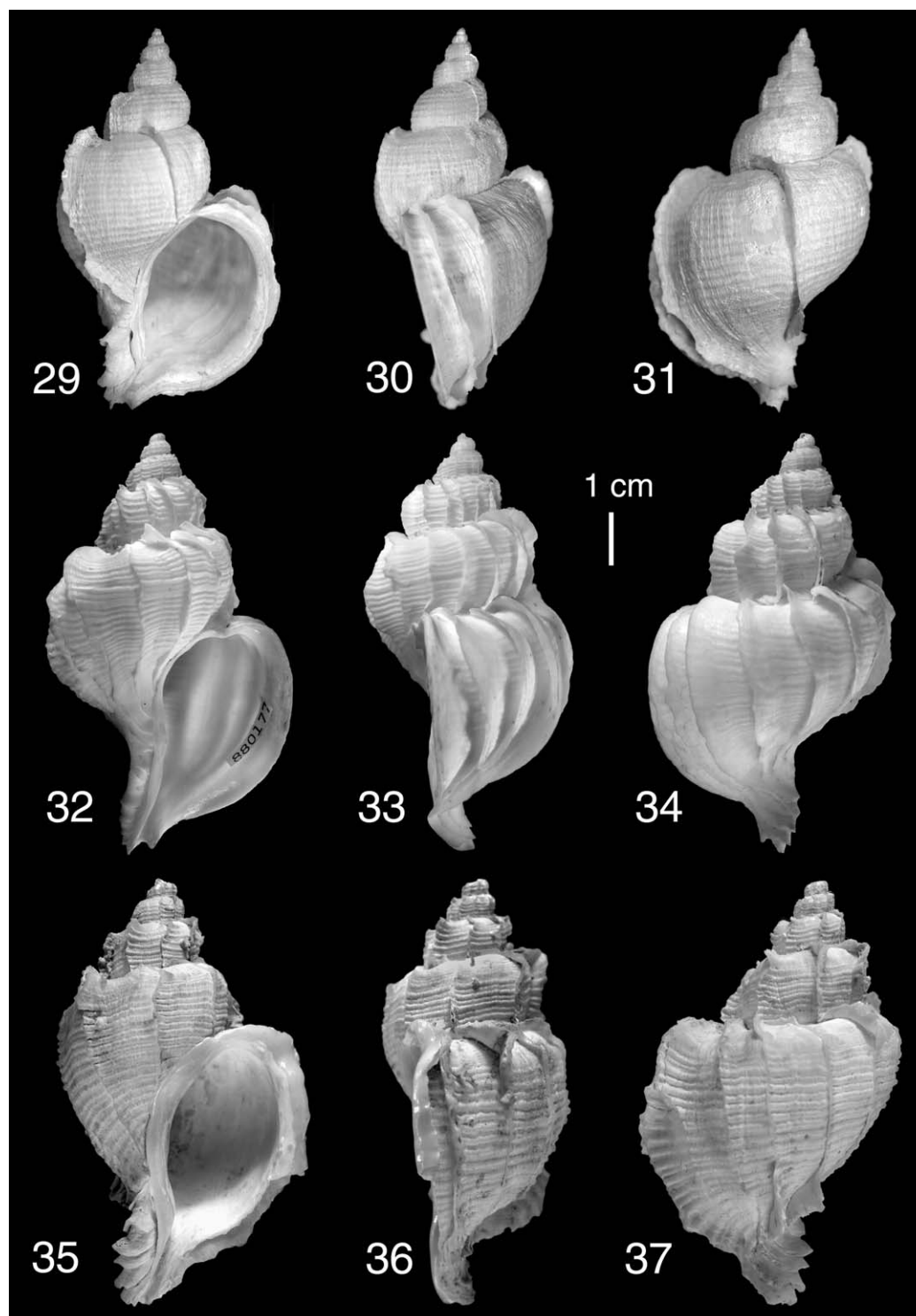
Figures 29–31. Trophonella enderbyensis (Powell, 1958). 29. Apertural, 30. lateral, and 31. dorsal views of the holotype, SAM D15497, off Enderby Land, Antarctica, 65°48'S, 71°24'E in 193 m. 32–34. Trophonella eversoni (Houart, 1997). 32. Apertural, 33. lateral, and 34. dorsal views of the holotype USNM 880177, South Atlantic Ocean, ? Antarctica, ? Kerguelen Is. 35–37. Trophonella rugosolamellata new species. 35. Apertural, 36. lateral, and 37. dorsal views of the holotype, ZMH 2777, off South Orkney Islands, 60°52.2'S, 44°28.4'W, in 205 m.
