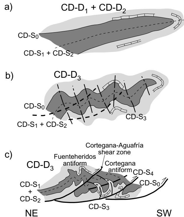
Fig. 4.- Schematic tectonic evolution proposed for the CD of the AMB (Díaz Azpiroz, 2001). a) As the result of the CD-D 1 and CD-D 2 deformation phases, km-scale recumbent folds and a high-temperature penetrative foliation (CD-S 2 ) were generated. b) CD-D 3 gave place to open symmetric upright folds. The discontinuous lines represent the localisation of the CD-D 4 shear zones. c) CD-D 4 produced km-scale thrusts, with a very penetrative mylonitic foliation (CD-S 4 ), and thrust accommodation folds (namely, the Fuentehieridos and the Cortegana antiforms).
