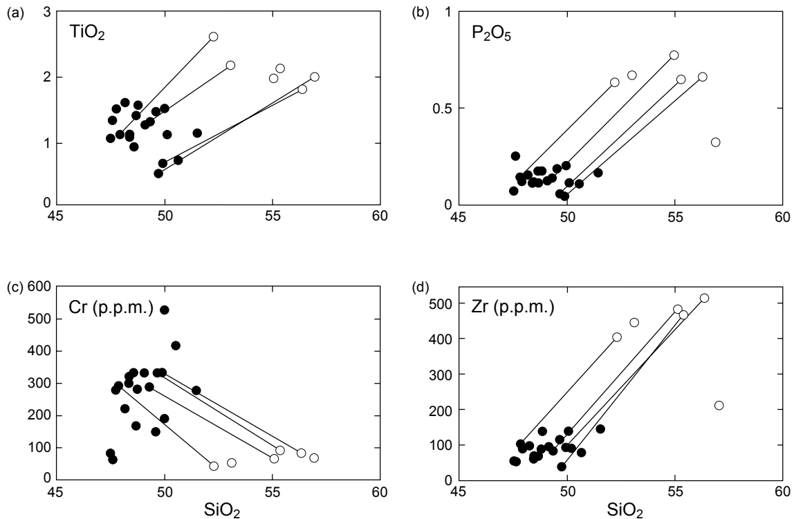
Fig. 12.- Silica variation plots for major and trace elements, showing the relationships between PI-Hb and quartz-rich amphibolites from the Acebuches series. Tie-lines link pairs of samples from two adjacent layers (from Castro et al. , 1996b).
