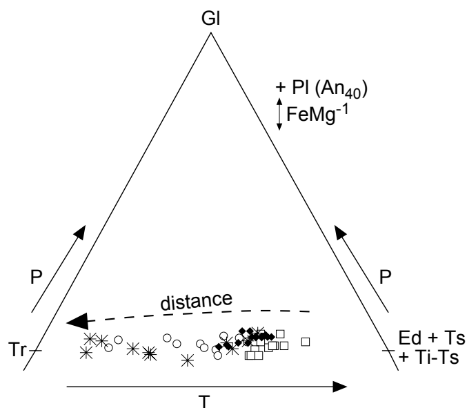
Fig. 8.- Qualitative thermobarometer (based on Castro et al. , 1996b) defined by a baricentric projection of amphiboles in the space Tr – GI – Ed + Ts + Ti-Ts, through the \text{FeMg}^{-1} interchange and from \text{PI}(\text{An}_{40}) . The curve marks the compositional evolution (with respect to the distance to the Calabazares shear zone) of the Acebuches amphiboles (symbols as in figure 7).
