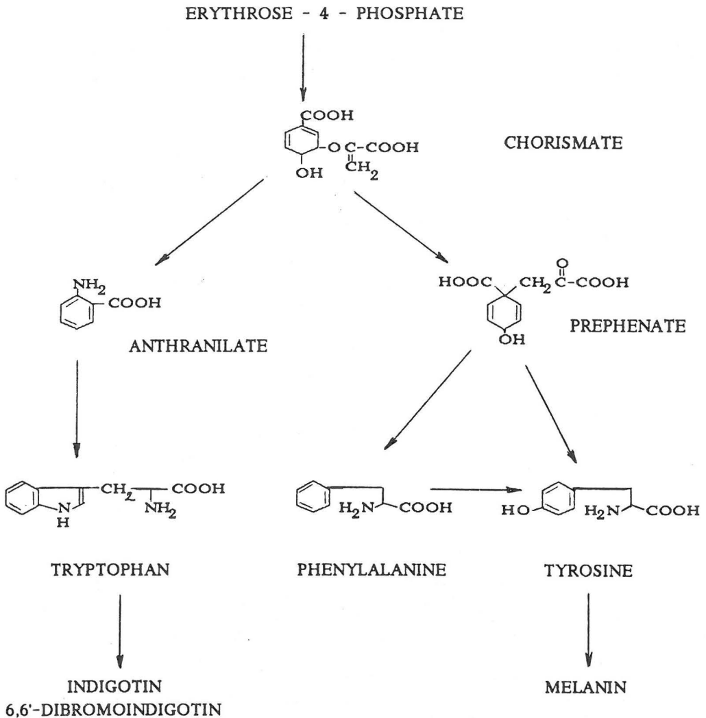
Fig. 2. — Biosynthesis of benzenoid aromatic amino acids.
