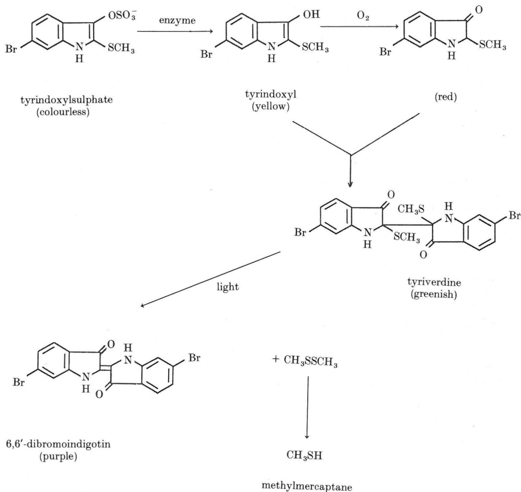
Fig. 4. — Formation of 6,6'-dibromoindigotin from tyrimdoxylsulphate.
