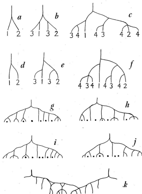
FIG. 1. a-c , Proboscoidactyla occidentalis ; d-f , P. circumsabella ; and g-k , P. flavicirrata , showing (diagrammatically) the branching of the radial canals. The numbers in figures a to f refer to the order of the canals and tentacles. The spots between the ends of the canal branches in figures g to j represent the position of tentacles to which no canals could be seen to be branching.
