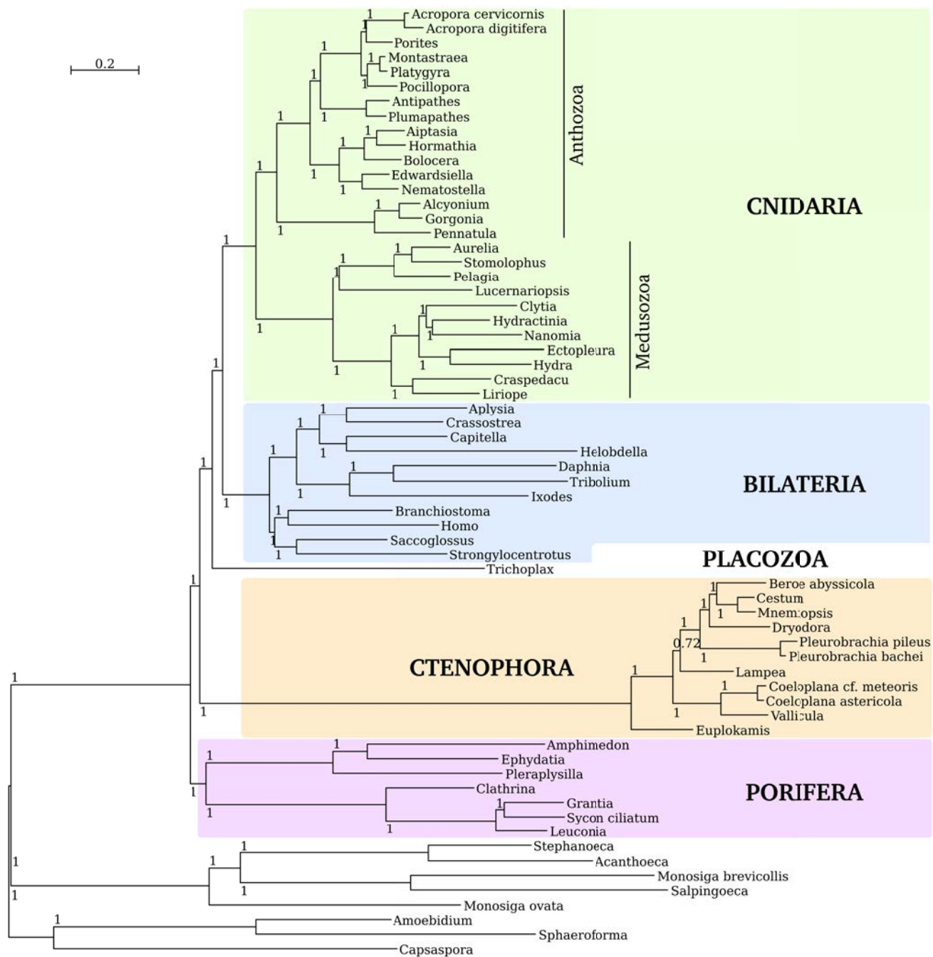
Figure 6: Phylogenetic relationships based on the AUTO-4235_65_PB60 matrix and reconstructed with CAT+T evolution model. Posterior probabilities of each branch are noted on the tree.
