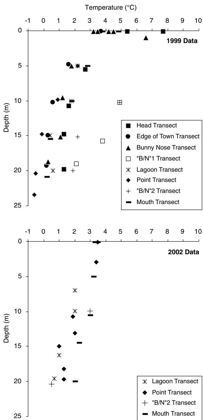
FIGURE 8. Water temperature values with depth along transects in Turton Bay in 1999 and 2002.
