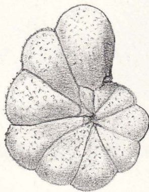
Avnimelech: Bathysiphon in Eocene of Israel Andersen: Haplophragmoides from Louisiana Coast
