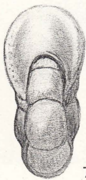
Avnimelech: Bathysiphon in Eocene of Israel Andersen: Haplophragmoides from Louisiana Coast
