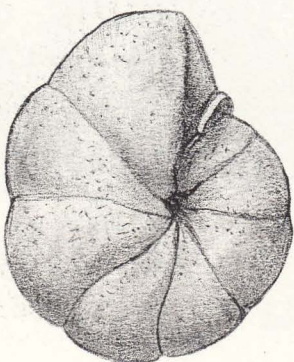
Avnimelech: Bathysiphon in Eocene of Israel Andersen: Haplophragmoides from Louisiana Coast
