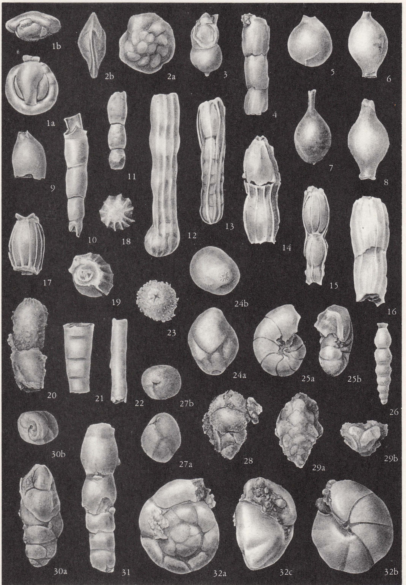
Todd: Tertiary Foraminifera from Amchitka Island
