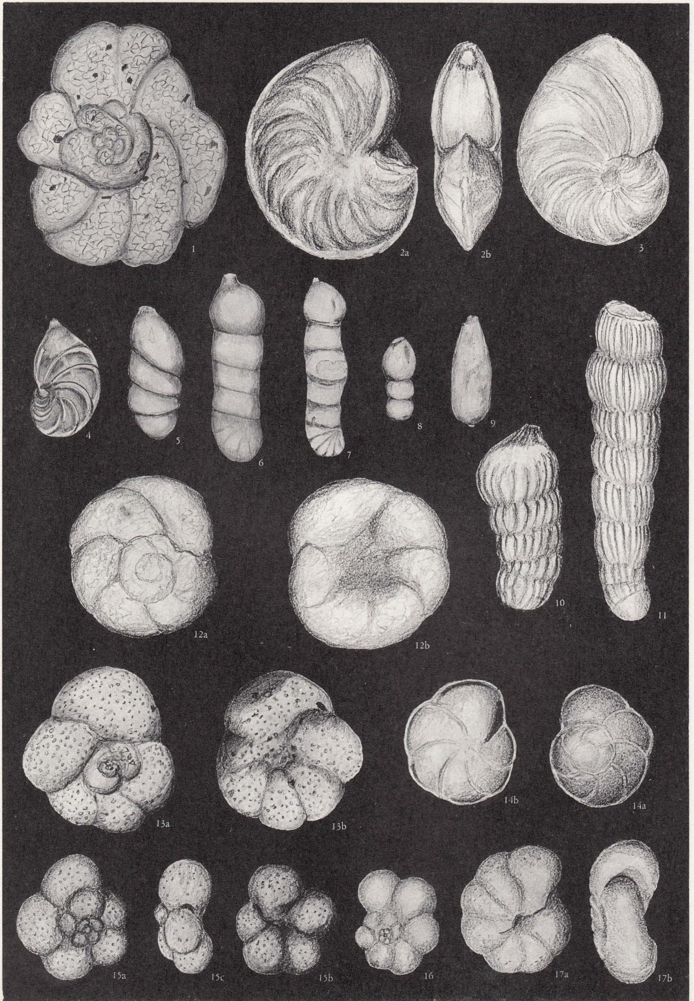
Crespin: Lower Cretaceous Foraminifera from Australia
