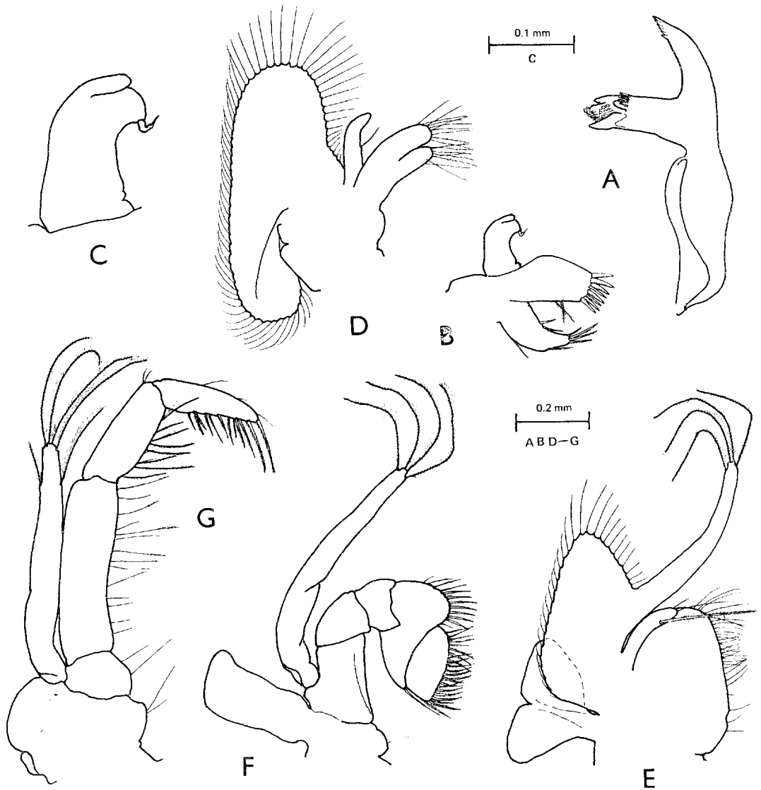
FIG. 5. — Periclimes ceratophthalmus Borradaile, ♂: A, mandible; B, maxillula; C, idem , palp; D, maxilla; E, first maxilliped; F, second maxilliped; G, third maxilliped.
