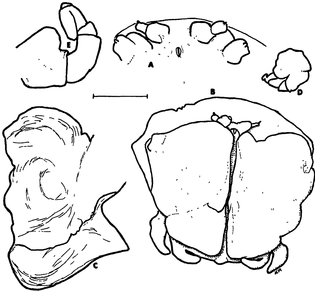
Fig. 29. Anuropodione carolinensis Markham, holotype female. A. Antennae. B. Head, ventral. C. Right oostegite 1, internal. D. Left pereopod 1. E. Right pereopod 7. Scale: 0.5mm for A; 0.1mm for B-E.
