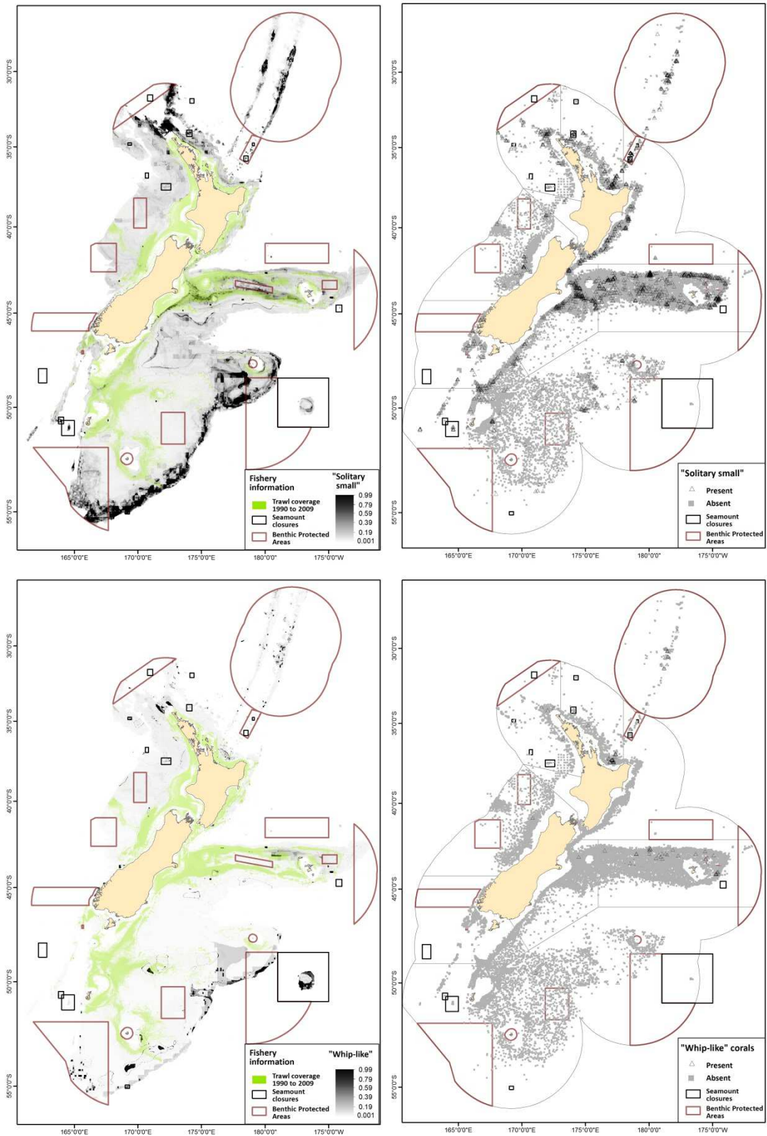
Figure D10: Predicted distributions (left) and location of coral presence/absence data records within the EEZ (right) for "solitary small" corals (upper) and "whip-like" corals (lower), relative to the 20-year trawl footprint (1989–90 to 2008–09) and seamount closures introduced in 2001 and Benthic Protected Areas introduced in 2007. FMAs of the EEZ are shown in Figure C2.
