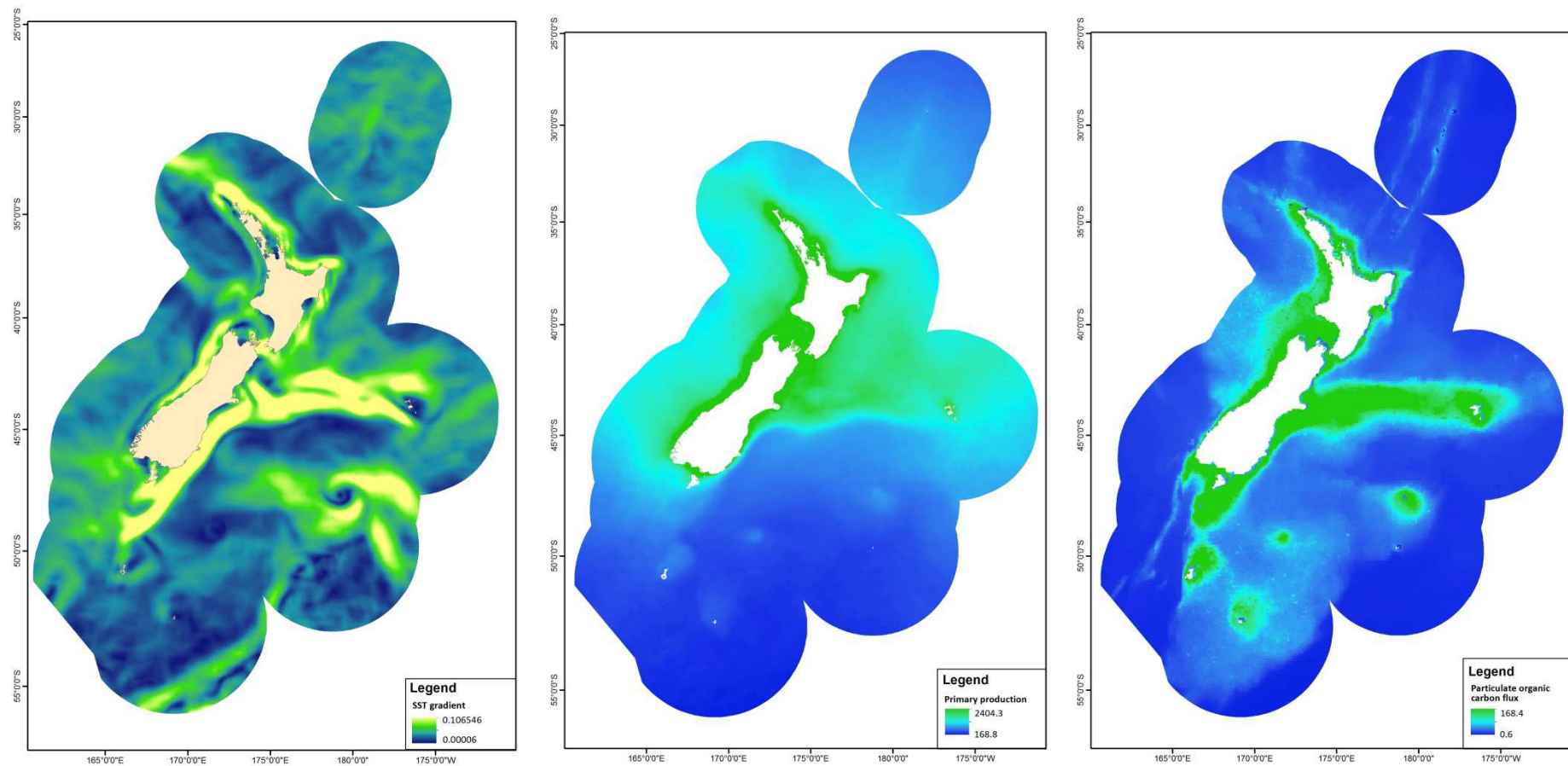
Figure B3: Distribution of environmental layers (on a 250 x 250 m grid) used in the predictive modelling: SSTgradient (left), surface water primary productivity ( \text{mg C m}^{-2} \text{d}^{-1} ) (centre), and particulate organic carbon flux (right).
