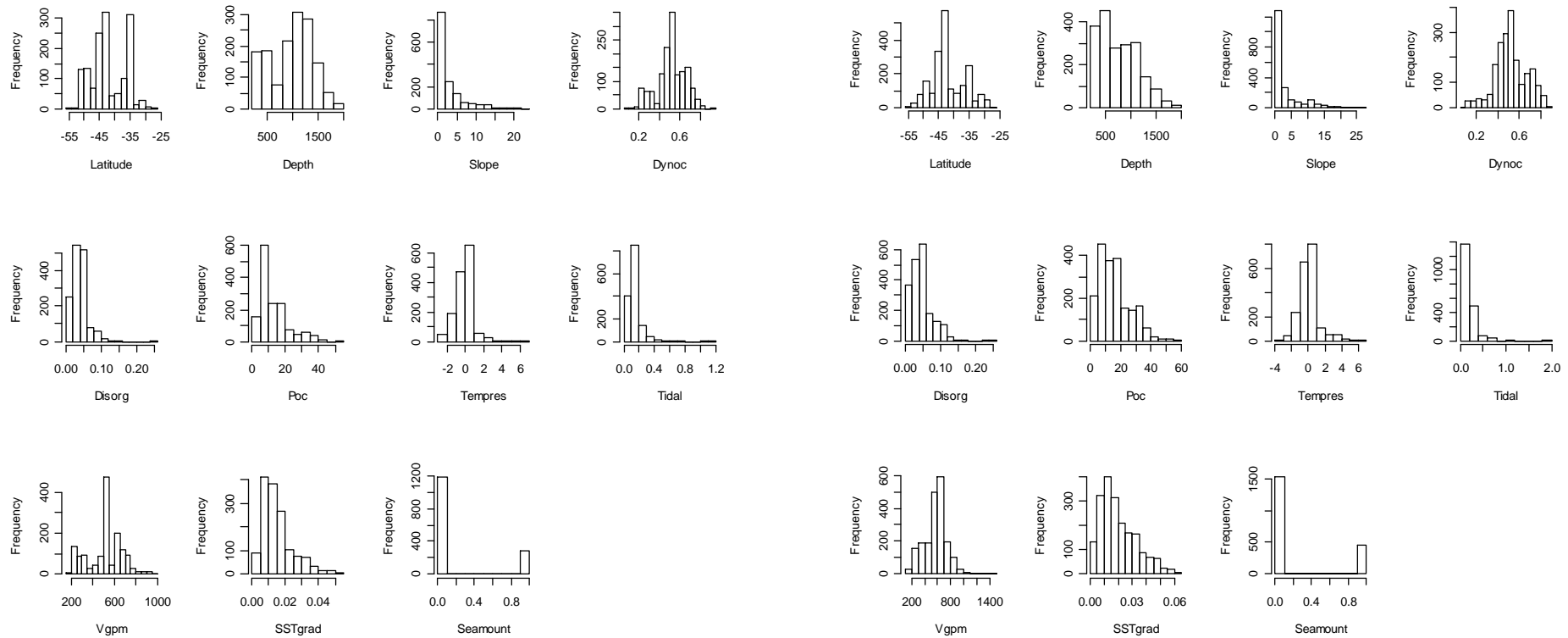
Figure D3: Frequency of “reef-like” corals (left) and “solitary small” corals (right), by latitude ( ^{\circ} S), depth (m), slope, dynamic topography, dissolved organic matter, particulate, bottom temperature residuals, tidal current, primary production, SST gradient, and underwater topographic feature (seamount). See Table C1 for units and description of environmental variables. See Table C1 for units and description of environmental variables.
