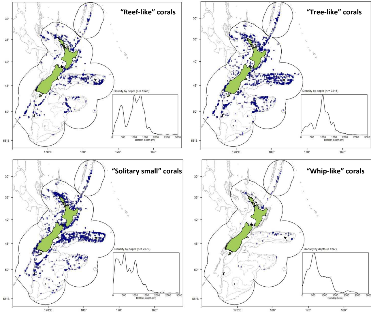
Figure C3: Location of coral records (o) and their depth distribution, within the New Zealand 200 n. mile EEZ, by the four functional groups. The 500 m, 1000 m, and 1500 m depth contours are shown.
