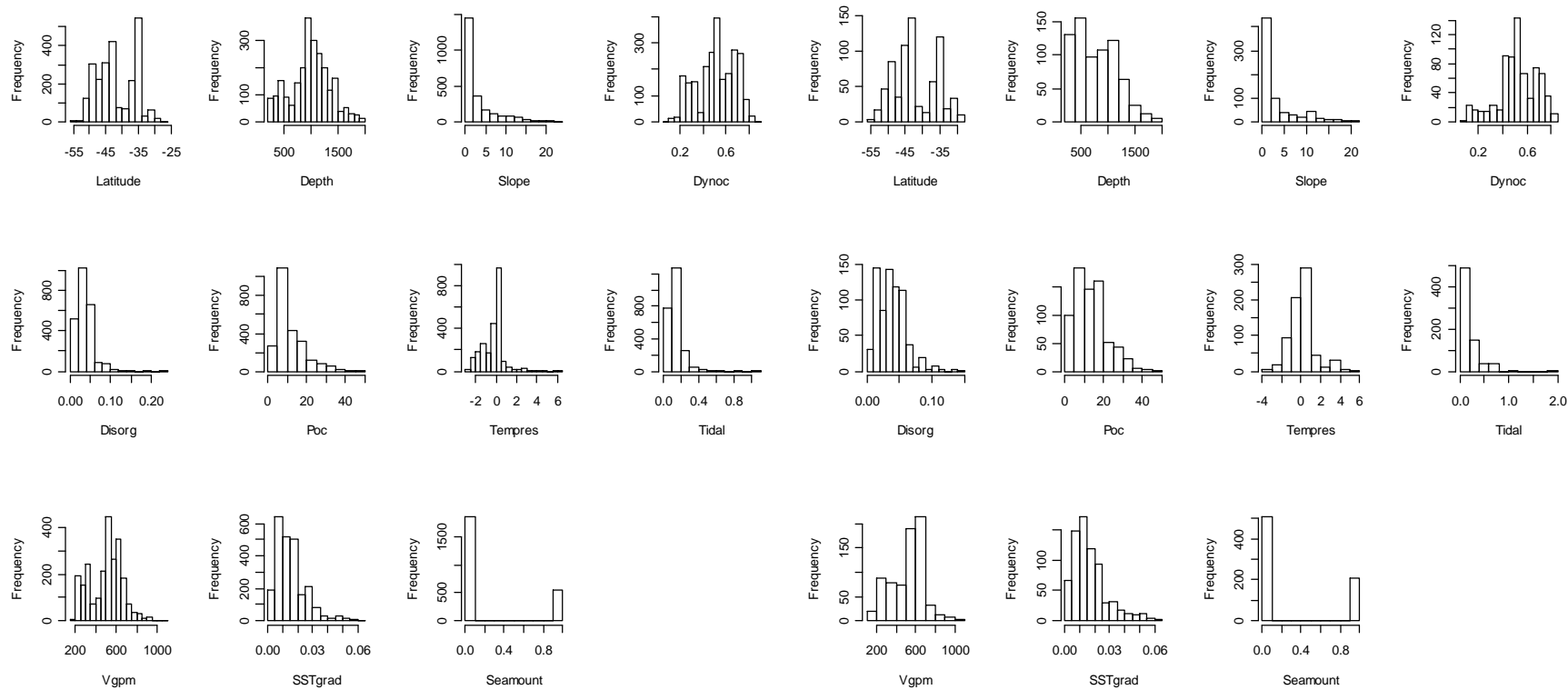
Figure D1: Frequency of gorgonian corals in Order Alcyonacea (left) and hydrocorals in Order Anthoathecata corals (right) in 200–2000 m, by latitude ( ^{\circ} S), depth, slope, dynamic topography, dissolved organic matter, particulate, bottom temperature residuals, tidal current, primary production, SST gradient, and underwater topographic feature (seamount). See Table C1 for units and description of environmental variables.
