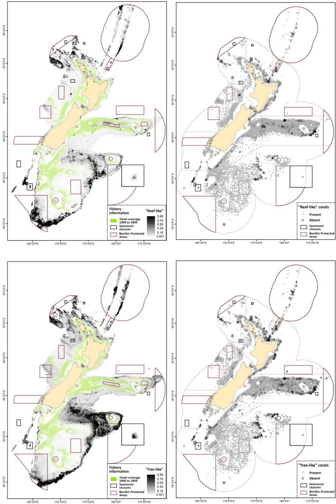
Figure D9: Predicted distributions (left) and location of coral presence/absence data records within the EEZ (right) for “reef-like” corals (upper) and “tree-like” corals (lower), relative to the 20-year trawl footprint (1989–90 to 2008–09) and seamount closures introduced in 2001 and Benthic Protected Areas introduced in 2007. FMAs of the EEZ are shown in Figure C2.
