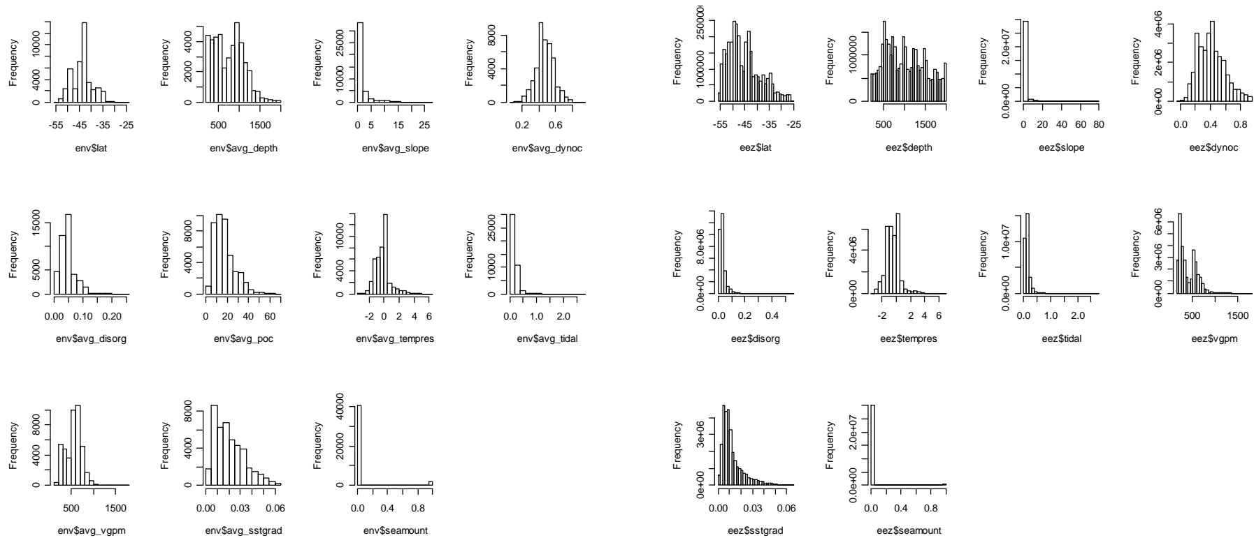
Figure D5: Frequency of benthic stations (left) and background EEZ 250 x 250 m cells (right) in 200–2000 m, by latitude (° S), depth (m), slope, dynamic topography, dissolved organic matter, particulate organic carbon flux, bottom temperature residuals, tidal current, primary production, SST gradient, and underwater topographic feature (seamount). See Table C1 for units and description of environmental variables.
