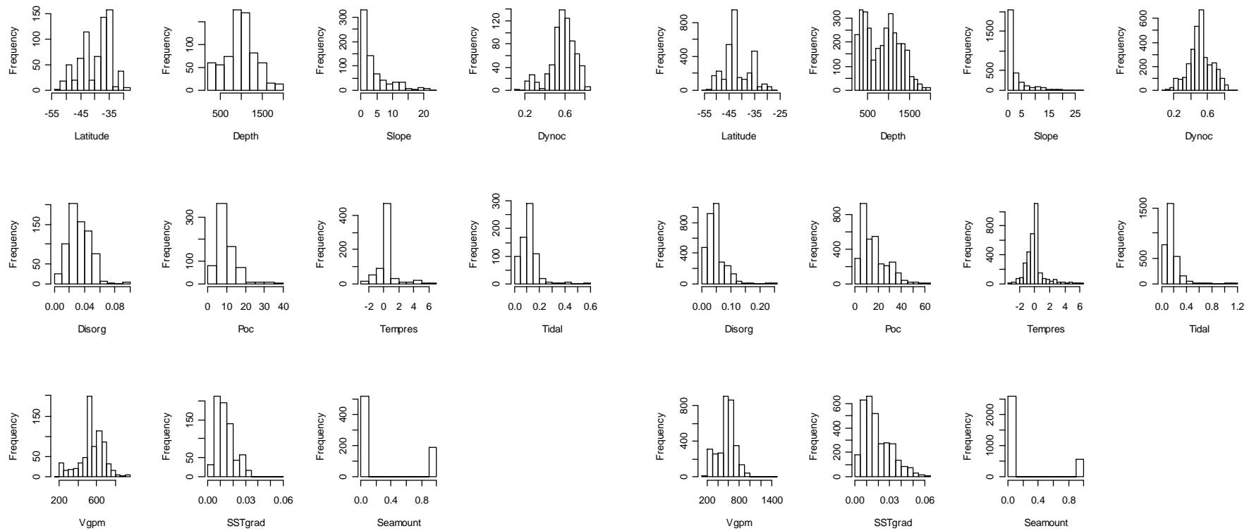
Figure D2: Frequency of black corals in Order Antipatharia (left) and stony corals in Order Scleractinia corals (right) in 200–2000 m, by latitude ( ^{\circ} S), depth, slope, dynamic topography, dissolved organic matter, particulate, bottom temperature residuals, tidal current, primary production, SST gradient, and underwater topographic feature (seamount). See Table C1 for units and description of environmental variables.
