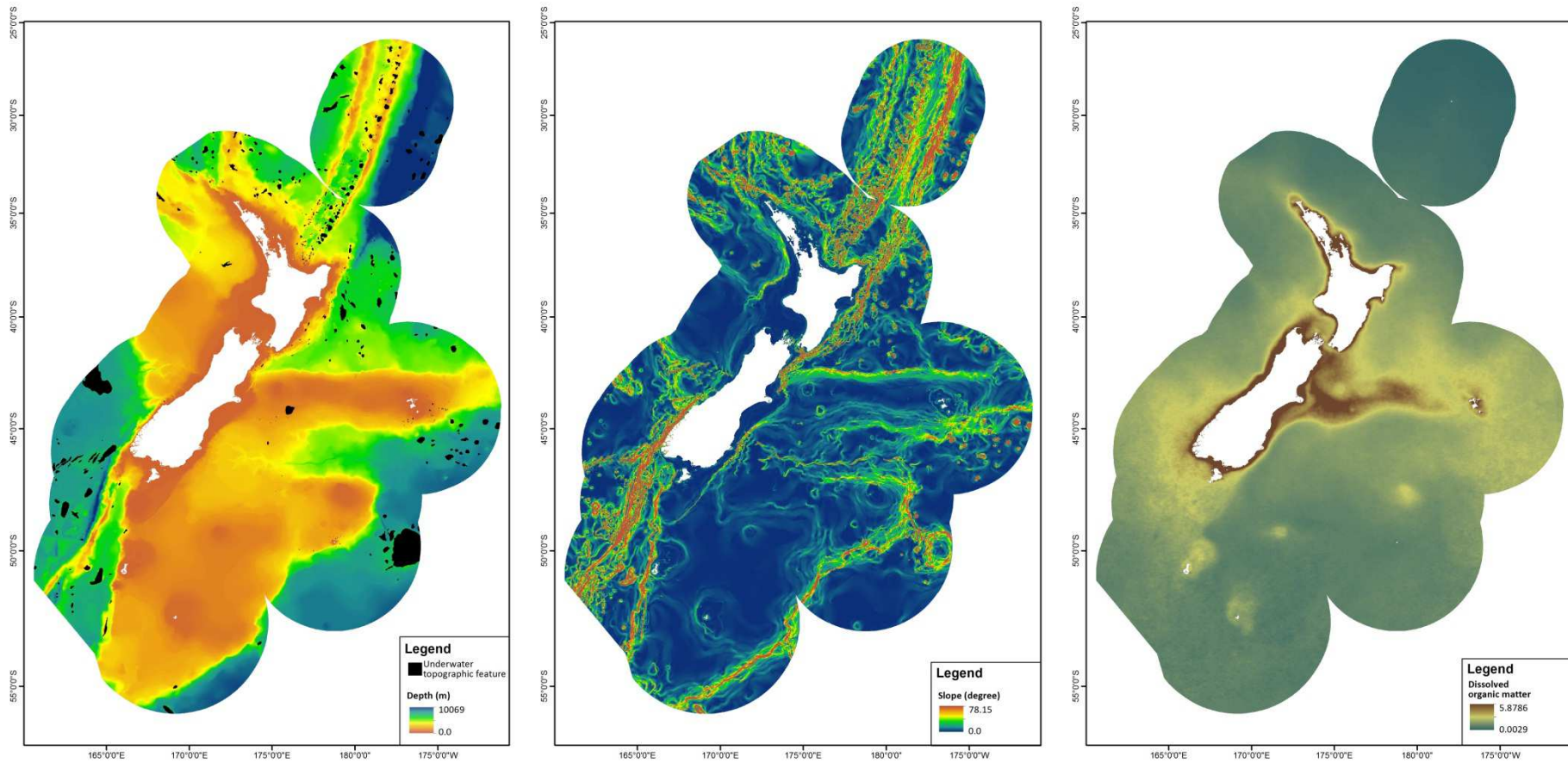
Figure B1: Distribution of environmental layers (on a 250 x 250 m grid) used in the predictive modelling: depth (m) and location of underwater topographic features (left), slope (°) (centre), and dissolved organic matter ( a_{\text{DOM}} (443) \text{ m}^{-1} ) (right).
