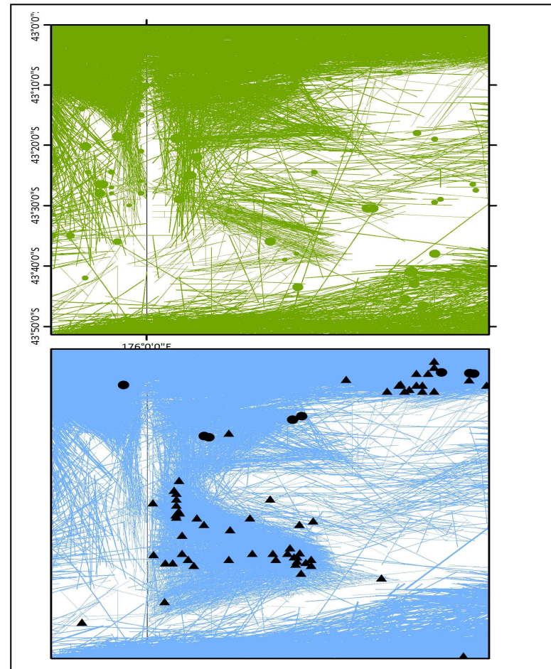
Figure E2: This represents a close-up of the area shown by the orange box on the Chatham Rise in Figure B2. The top box shows the 1989–90 to 2004–05 trawl footprint (Baird et al. 2011, Baird & Wood 2012) in this area southeast of the Mernoo Bank. The lower plot shows the 1989–90 to 2008–09 trawl footprint (GNS 2012) and includes locations of observed coral catches, for data that match the top footprint (●) and for observed coral data collected since October 2005 (▲).
