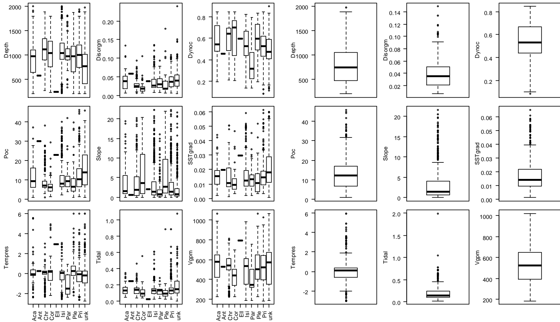
Figure D6: Distribution of environmental variables by gorgonian family in Order Alyconacea (left) and by Family Stylasteridae in Order Anthoathecata (right). See Table C1 for variable name and units and Table A3 for full family names.
