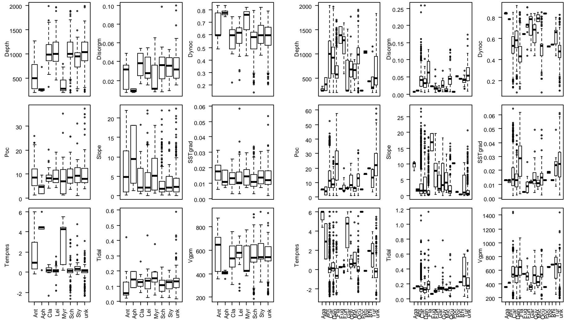
Figure D7: Distribution of environmental variables by family in Order Antipatharia (left) and by family in Order Scleractinia (right). See Table C1 for variable name and units and Table A3 for full family names.
