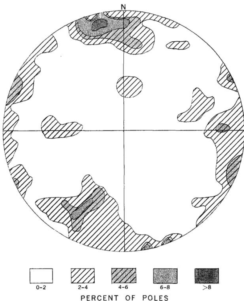
FIGURE 3.—Contour diagram of poles of 127 joints measured in the Tye Lake powersite area. Poles plotted on lower hemisphere. Contoured on percent of poles. (Billings, 1954, p. 108-114.)
