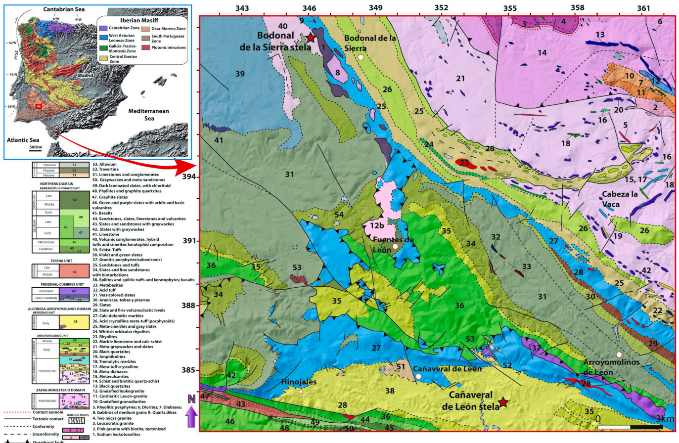
Fig. 3. Left: Synthetic geological map of Iberian Peninsula after the “Geological map of Spain with the inclusion of continental Portugal. Scale: 1:2.000.000 (Vera, 2004); Right: Geological map of the study area, modified from the Instituto Geológico y Minero de España (IGME). The geology is overlain on a digital terrain model based on public domain data by the Centro Nacional de Información Geográfica. The red stars correspond to the location of the Cañaverel de León and Bodonal de la Sierra stelae. Design: José Antonio Lozano Rodríguez.
