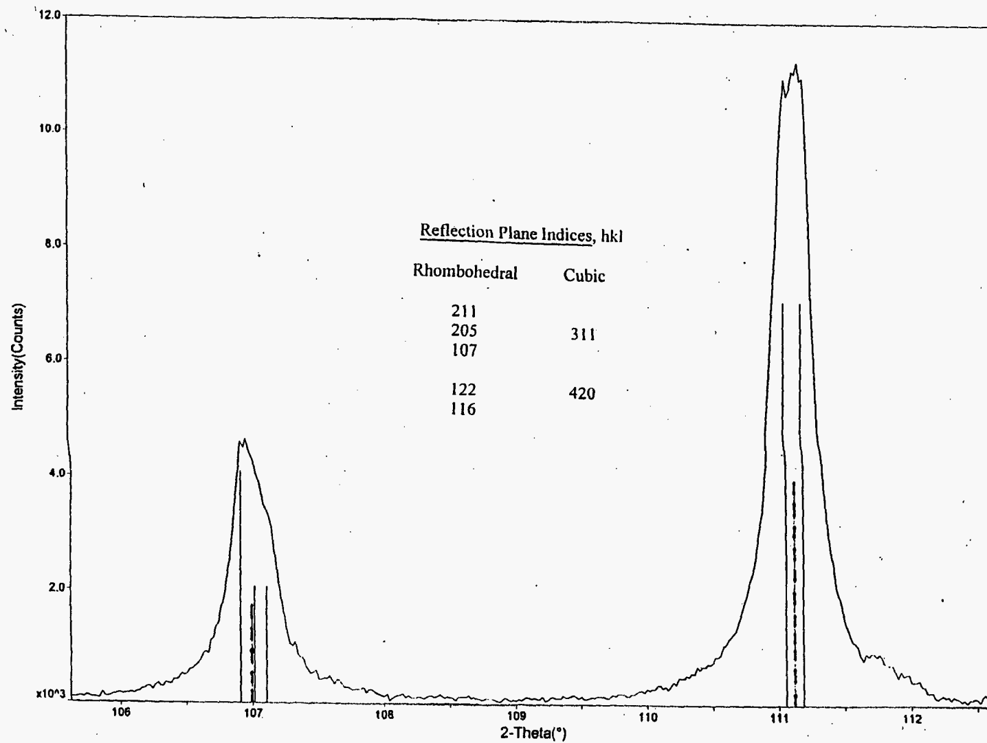
Fig. 1. Comparison of higher angle X-ray diffraction peaks for coarsened NiO with lines for rhombohedral (—) and cubic (----) nickel(II) oxide; copper K_{\alpha} radiation.
