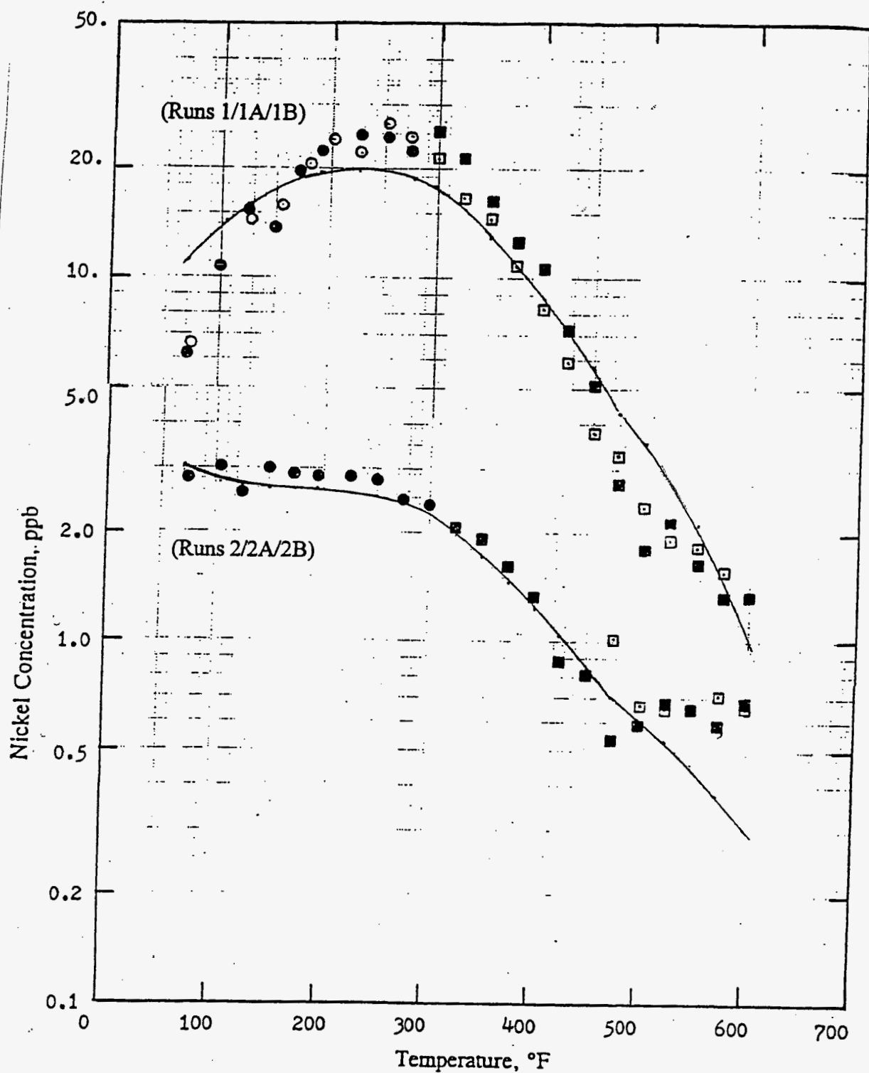
Fig. 3. Comparison of measured and predicted solubilities of (hydrated) nickel(II) oxide in aqueous ammonium hydroxide: Runs 1/1A/1B, \text{NH}_3 \approx 0.07 mm; Runs 2/2A/2B, \text{NH}_3 \approx 0.7 mm.
