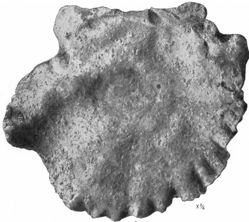
PLIOCENE FOSSILS FROM LIMESTONE IN SOUTHERN FLORIDA
