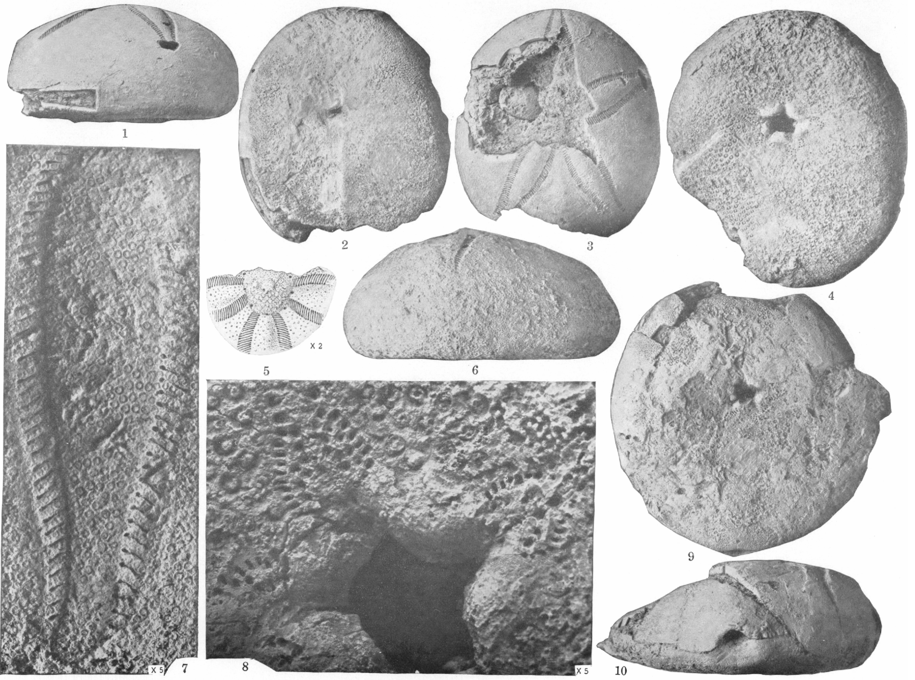
PLIOCENE FOSSILS FROM LIMESTONE IN SOUTHERN FLORIDA
