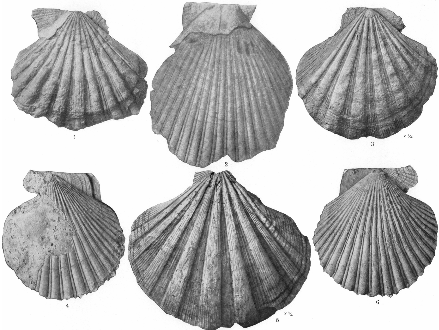
PLIOCENE FOSSILS FROM LIMESTONE IN SOUTHERN FLORIDA Shows also, for comparison, specimens obtained elsewhere
