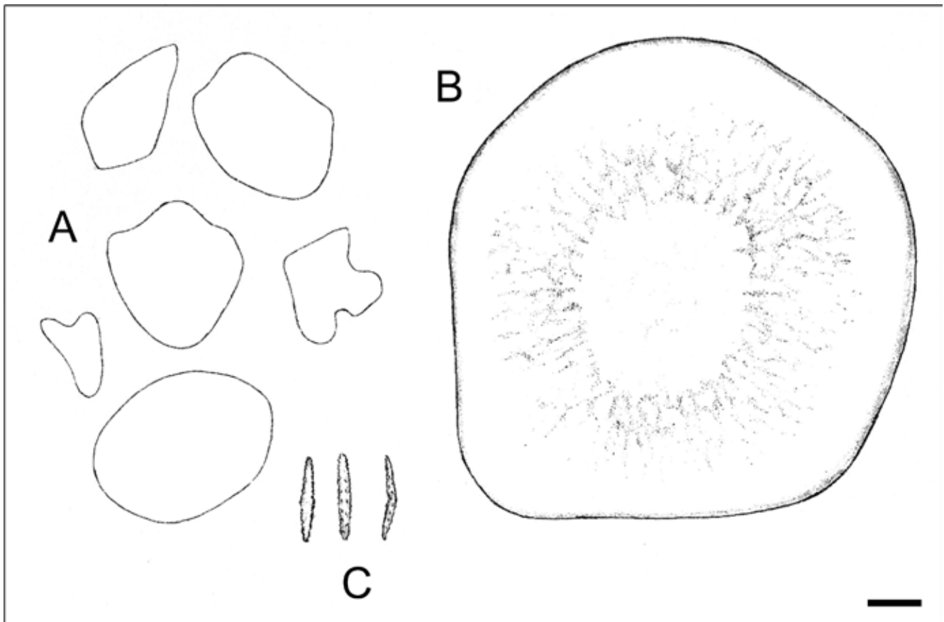
Figure 19. Lepidothenea incrustans (Dendy, 1924)
