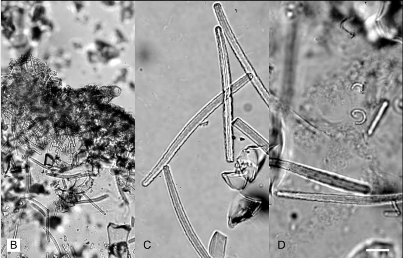
Figure 26. Scleroderma flabelliformis Sollas, 1888.
