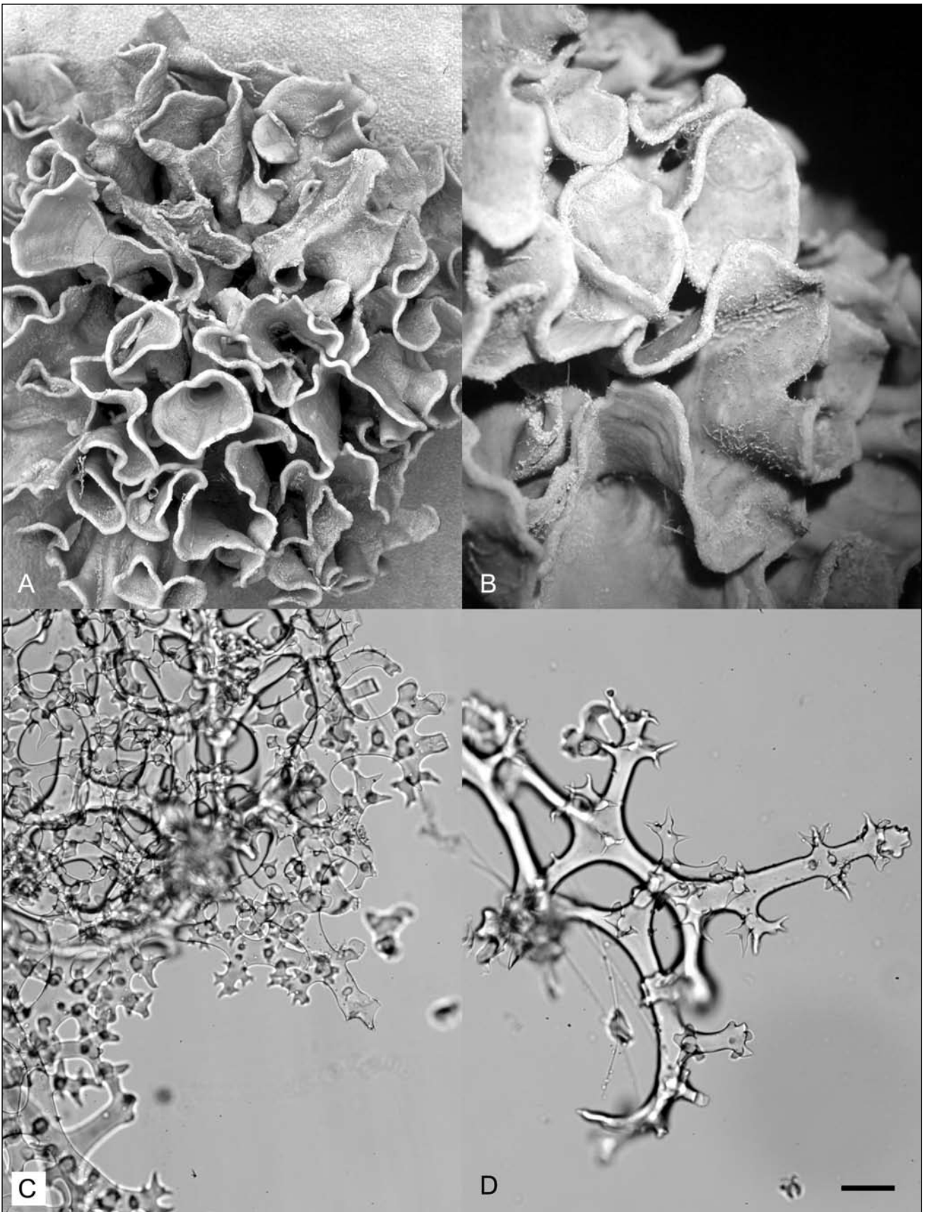
Figure 31. Leiodermatium intermedia (Sollas, 1888)
