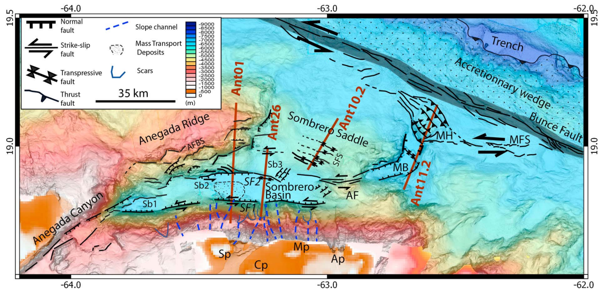
Figure 5. Interpretation of multibeam data in the northern Lesser Antilles margin. AF: Anguilla Fault, Ap: Anguilla Platform, AFBS: Aneгада Faults and Basin System, Cp: Crocus Platform, MB: Malliwana Basin, MFS: Malliwana Faults System, MH: Malliwana Hill, Mp: Malliwana Platform, Sb1-Sb2-Sb3: three Sombrero subbasins. Sp: Sombrero platform.
