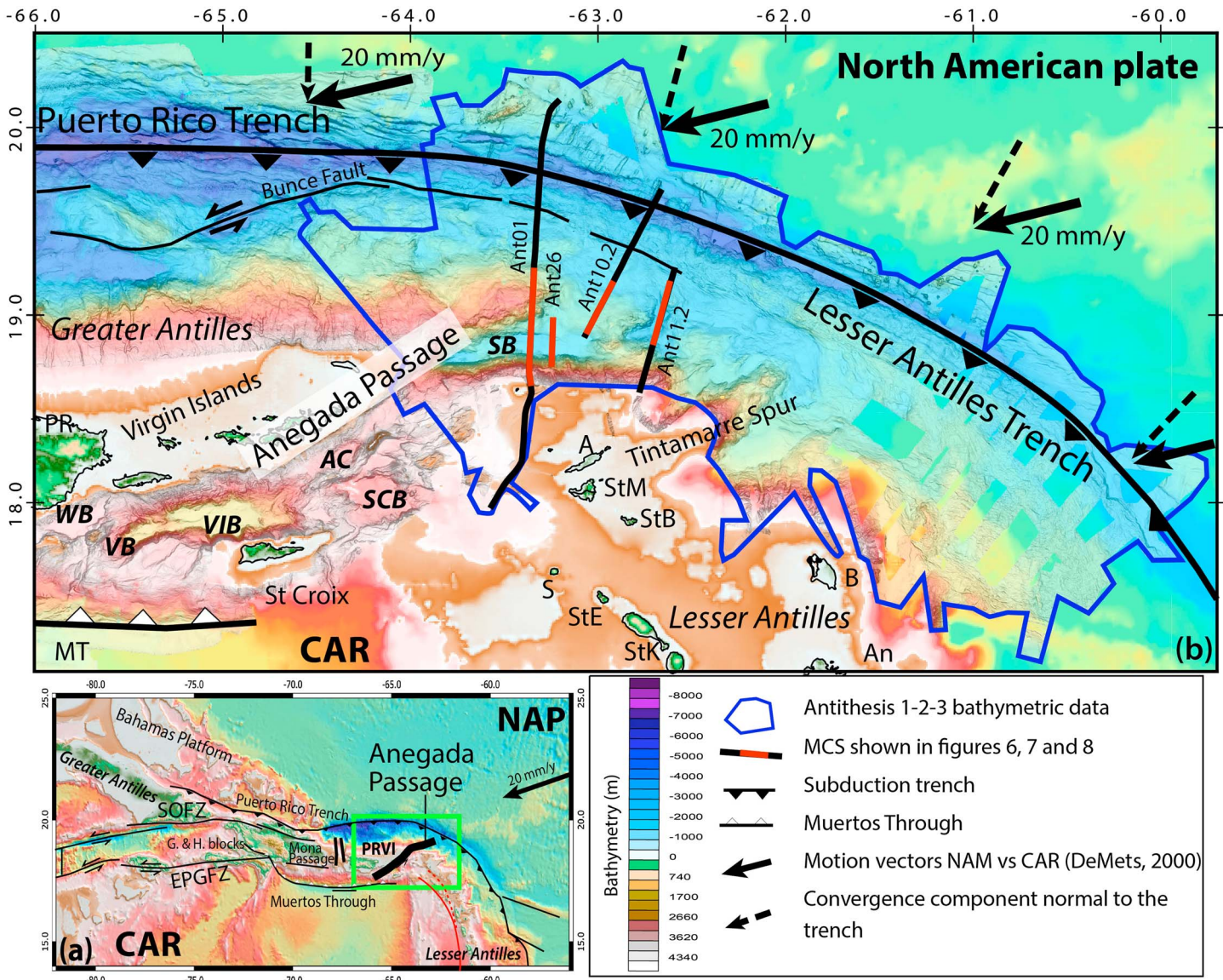
Figure 1. Bathymetric maps showing the geodynamic and tectonic settings of (a) the Caribbean Plate [Leroy et al., 2015; Corbeau et al., 2016] and (b) the Anegada Passage. The bathymetry is a compilation of data acquired during the Antithesis cruises (100 m grid resolution), data acquired during eight surveys between 2002 and 2013 [Andrews et al., 2013] (150 m grid resolution) and Smith and Sandwell [1997] altimetry-derived data (1' grid resolution). Plain and dotted black arrows stand for convergence vector between the North American and the Caribbean Plates [DeMets et al., 2000] and convergence component normal to the trench, respectively. Note that the length of dotted arrows is not representative to the normal convergence component slip. The convergence obliquity increases northward. Green and blue contours, respectively, frame the study area for this paper in Figure 1a and for the Antithesis cruises in Figure 1b. A: Anguilla; An: Antigua; AC: Anegada Canyon/Anegada Passage (sensu stricto); B: Barbuda; CAR: Caribbean Plate; G&H: Gonave and Hispaniola; PR: Puerto Rico; S: Saba; SB: Sombrero Basin; SCB: St Croix Basin; StB: St Barthélemy; StE: St Eustace; StK: St Kitts; StM: St Martin; VB: Vieques Basin; VIB: Virgin Island Basin; and WB: Whiting Basin.
