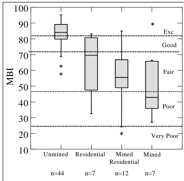
Figure 17. Boxplot of MBI scores among landuse types.
