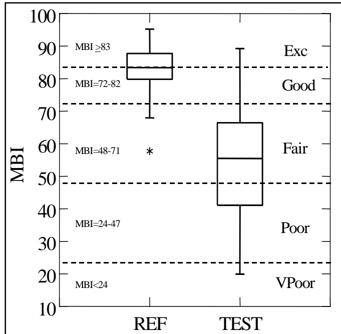
Figure 12. Box plot of MBI scores from reference and test sites (all sites) showing thresholds for narrative ratings.
