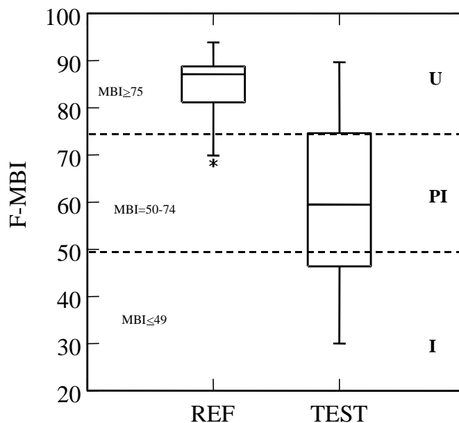
Figure 19. Box plot of F-MBI scores from reference and test sites (all sites) showing thresholds for use-support designations. U=Unimpaired, PI=Partially Impaired, I=Impaired.
