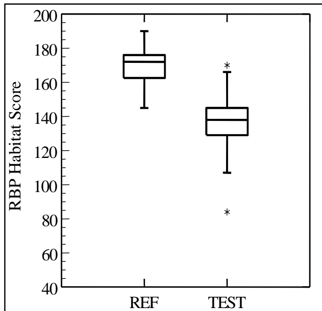
Figure 13. Box plot of RBP habitat scores from reference and test sites (2000-2002).
