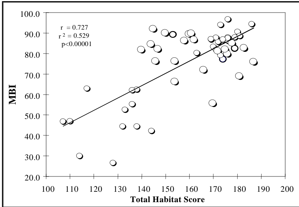
Figure 14. Relationship of MBI to Total Habitat Score (2000-2001 sites).
