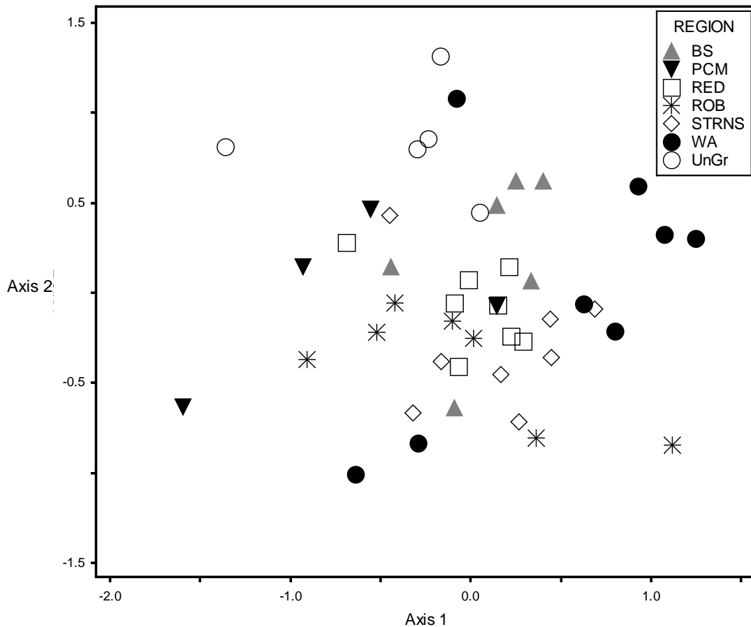
Figure 7. NMDS ordination (genus level) of all reference sites grouped by geographic region. ROB=Robinson Forest, RED=Redbird Ranger District, STRNS=Stearns Ranger District, PCM=Pine/Cumberland Mountains, BS=Big Sandy, WA=Western Allegheny and UnGr=Un- Grouped.
