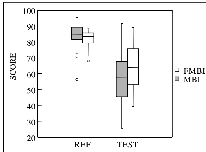
Figure 20. Box plot of MBI and Family-level MBI (F-MBI).
