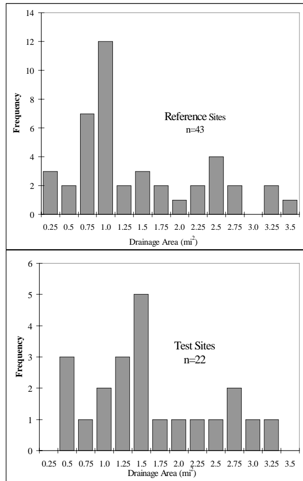
Figure 2. Distribution of reference and test sites by drainage area. Duplicate sample events excluded.
