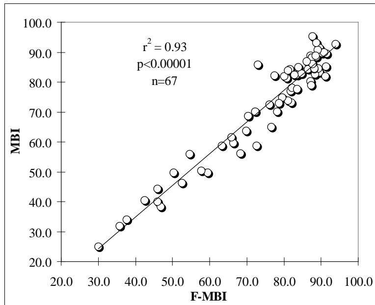
Figure 18. Relationship of Original MBI scores to the Family-level MBI (F-MBI)
