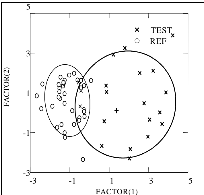
Figure 5. Discriminant root scores using %embeddedness, conductivity, canopy, and total habitat score (2000-2001 data).
