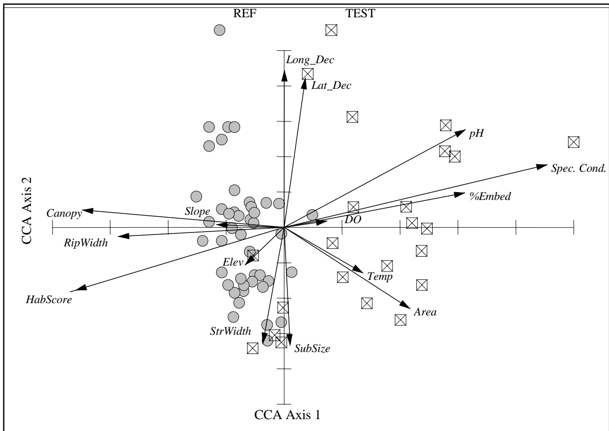
Figure 8. Canonical Correspondence Analysis (CCA) of all reference and test sites.
