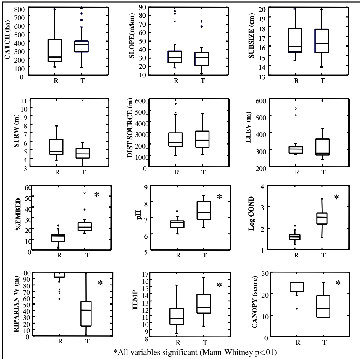
Figure 6. Box plots of selected environmental variables from reference and test sites (2000 calibration data).
