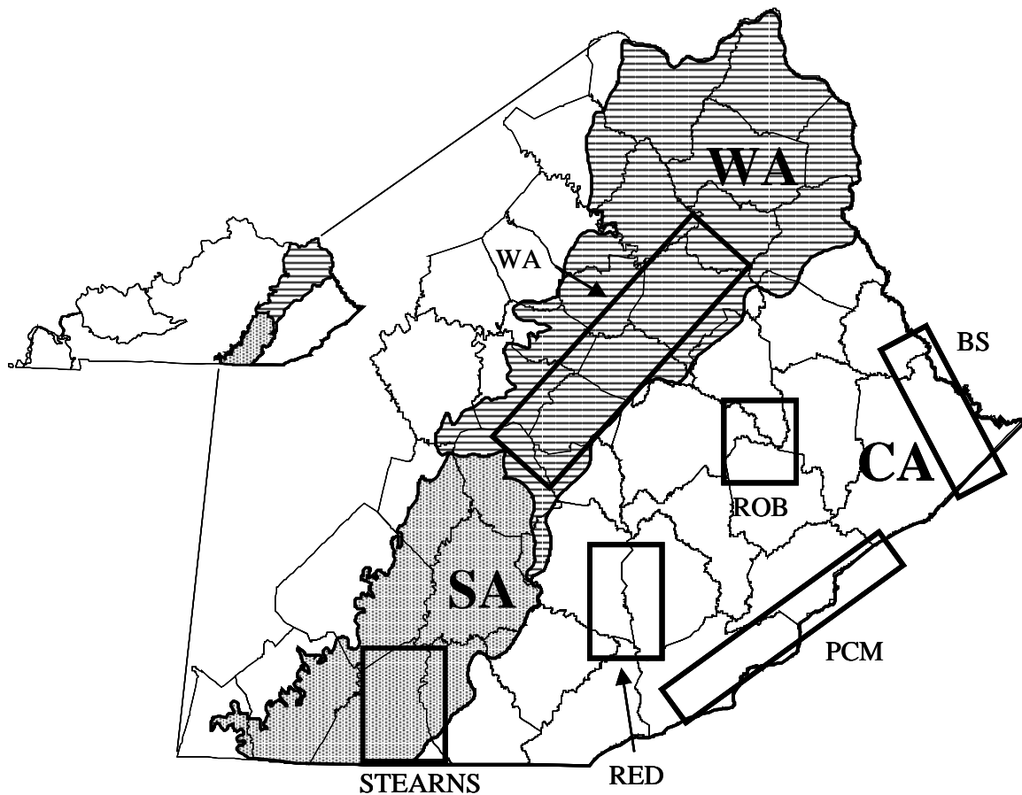
Figure 1. Generalized map of the 6 sampling areas showing ecoregions found within the Eastern Coalfield Region. CA=Central Appalachians, SA=Southwestern Appalachians, WA= Western Allegheny. See text for sampling area descriptions.
