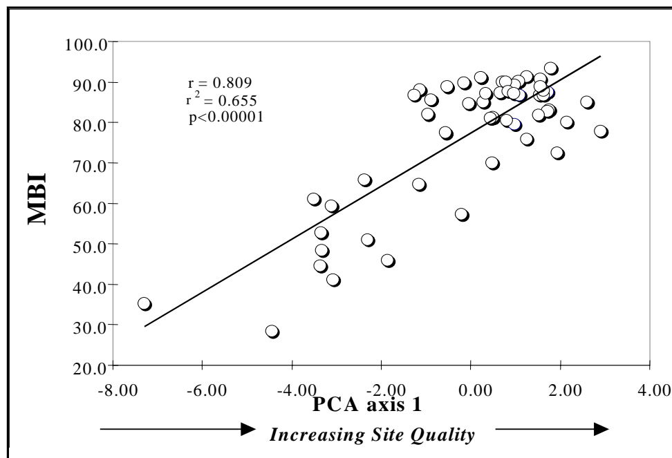
Figure 15. Relationship of the MBI to a perceived disturbance gradient as defined by PCA axis 1 (2000-2001 sites).
