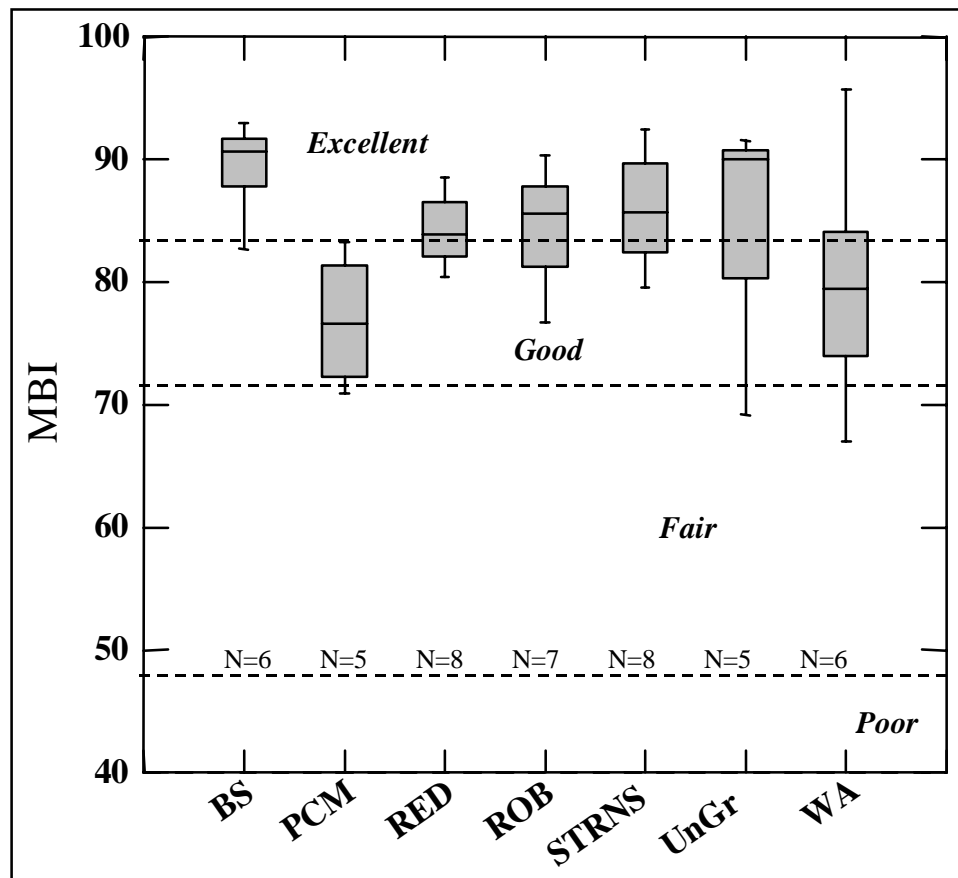
Figure 16. Box plot of reference MBI scores among study regions. Narrative ratings delineated by dashed lines. BS=Big Sandy, PCM=Pine/Cumberland Mountains, RED= Red-bird District, ROB=Robinson Forest, STRNS=Stearns District, UnGr=UnGrouped, WA=Western Allegheny.
