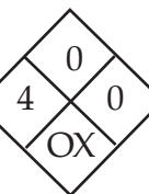
nitric acid
