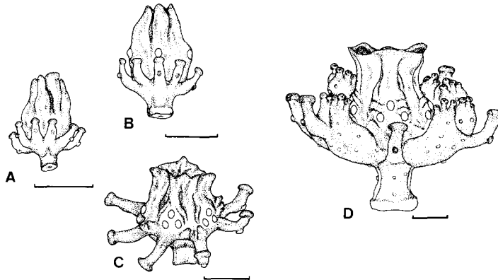
Fig. 10. Sasakiella cruciformis . Early metamorphosis. (A), juvenile with only eight primary tentacles; (B), ditto with one white spot on the manubrium in each perradius; (C), ditto with a pair of swellings at the base of manubrium; (D), ditto with three secondary tentacles at the tip of each arm. Bars represent 0.5 mm.
