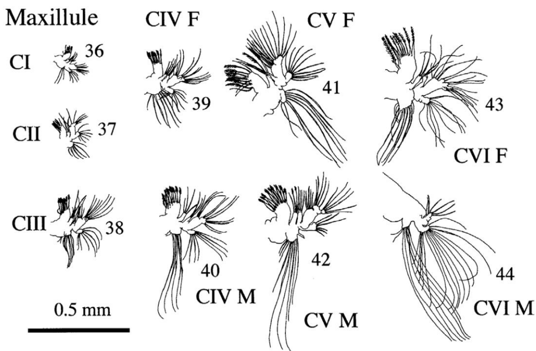
Figs 27-44. Gaetanus variabilis (Brodsky, 1950). 27-35, mandible: copepodid stage I (CI), CII, CIII, CIV female (CIV F), CIV male (CIV M), CV F, CV M, CVI F, and CVI M; 36-44, maxillule: CI, CII, CIII, CIV F, CIV M, CV F, CV M, CVI F, and CVI M.
