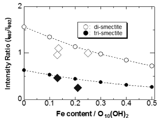
Fig.8. XRD intensity ratios of basal reflections ( I_{003}/I_{002} ) vs. Fe contents of tri- and di-smectite based on XRD modeling by Newmod (Reynolds, 1985). The measured values of tri-smectite (◆) and di-smectite (◇) from the Hishikari deposits (see Table 2) are plotted.
