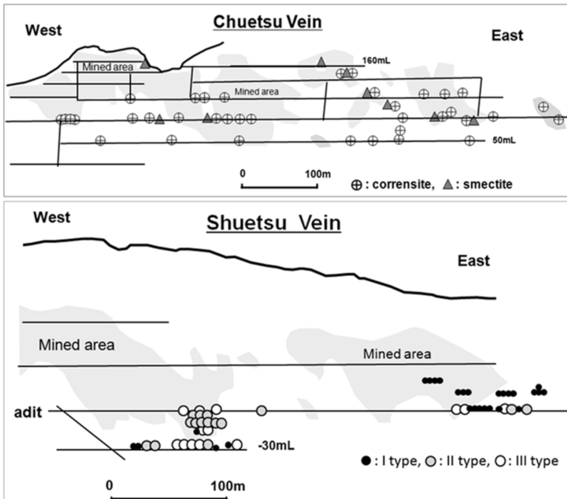
Fig.5. Distribution of corrensite, smectite and Co-C minerals (types of I-III) in the Chuetsu vein (upper) and the Shuetsu vein (lower) of the Todoroki deposit.
