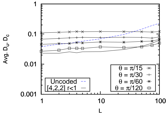
FIGURE 15. Experimental results from the ibmq_Jakarta device showing random sequences of the [4, 2, 2] -encoded gates and of the corresponding uncoded gate for sequence lengths L . A rotation error \theta is inserted after the Hadamard gate in the encoding circuit. 30 samples 21.06.2021
