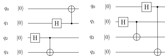
FIGURE 18. Encoder for |\overline{0+}\rangle
