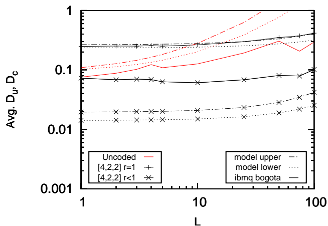
FIGURE 14. Experimental results based on the ibmq_Bogota device characterizing random sequences of the [4, 2, 2] -encoded gates and the corresponding uncoded gate for sequence lengths L . Model parameters: samples = 60, date= 15.04.2021, Gate set = [X_0, X_1, Z_0, Z_1, cz_{0,1} \circ Z_0 Z_1, H_0 H_1 \circ SWAP_{0,1}] , P_m = 0.04 , \epsilon_1 : \epsilon_2 = 1 : 50 , 3 \times 10^{-3} < \epsilon_1 < 5 \times 10^{-3} .
