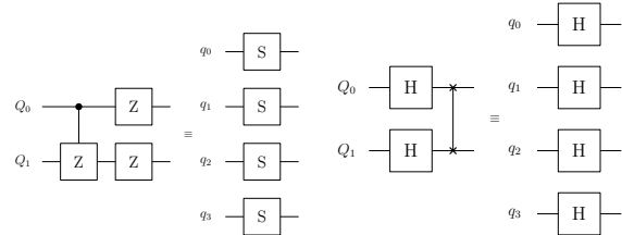
FIGURE 9. cz_{0,1} \circ Z_0 Z_1 Circuit
