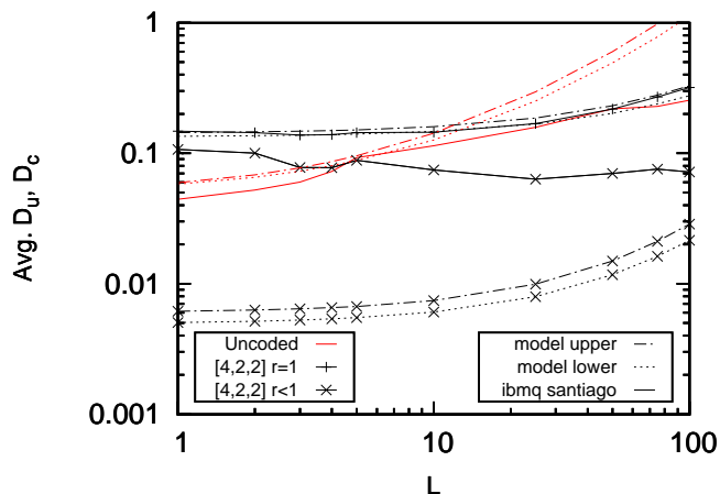
FIGURE 13. Experimental results based on the ibmq_Santiago device characterizing random sequences of the [4, 2, 2] -encoded gates and the corresponding uncoded gate for sequence lengths L . Model parameters: samples = 58, date= 14.02.2021, gate set = [X_0, X_1, Z_0, Z_1, cz_{0,1} \circ Z_0 Z_1, H_0 H_1 \circ SWAP_{0,1}] , P_m = 0.025 , \epsilon_1 : \epsilon_2 = 1 : 20 , 5 \times 10^{-3} < \epsilon_1 < 6 \times 10^{-3} .
