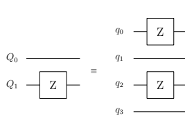
FIGURE 8. Z_1 Circuit
