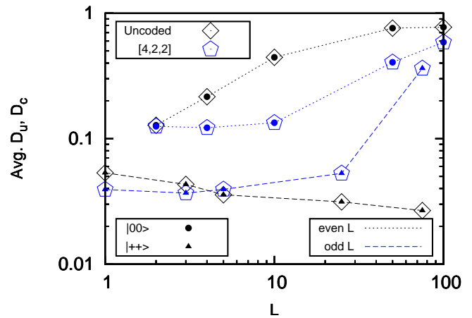
FIGURE 12. Experimental results based on the Ibmq_Santiago device characterizing the [4, 2, 2] -encoded H_0H_1 \circ SWAP_{0,1} gate repeated for the gate sequence lengths L . The final state at the circuit output is either |00\rangle (1-dimensional) or |++\rangle (4-dimensional), which are both denoted by different symbols.
