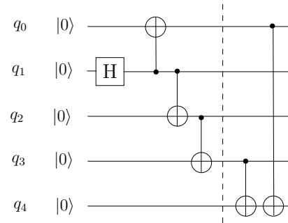
FIGURE 6. Fault-tolerant circuit to prepare the [[4, 2, 2]] -encoded logical state |\overline{00}\rangle . After the dashed line a parity check of (q_0, q_3) is determined by measuring the ancilla in q_4 . To make this circuit fault-tolerant post-selection is also applied to q_0 to q_3 .
