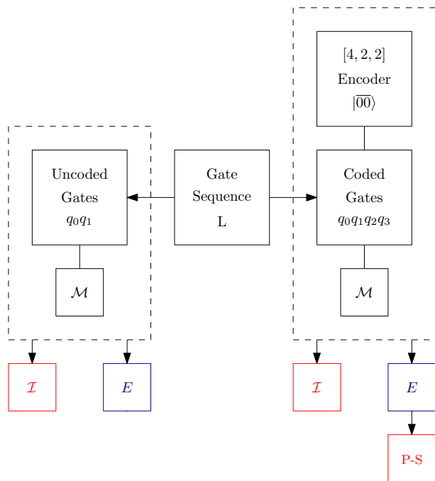
FIGURE 3. Schematic of the experiments design where \mathcal{M} denotes a quantum measurement. Furthermore, the red boxes indicate that the outcome is derived classically and the blue boxes represent a quantum experimental result. Finally, \mathcal{I} and \mathcal{E} are the ideal and the experimental outcome distribution, respectively, while P-S denotes classical post-processing.
