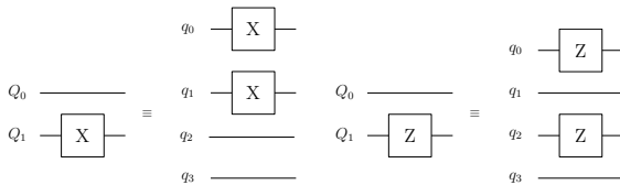
FIGURE 7. X_1 Circuit
