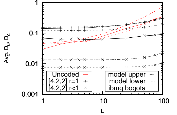
FIGURE 11. Experimental results based on the Ibmq_Bogota device characterizing random sequences of the [4, 2, 2] -encoded gates along with those of the corresponding uncoded gate for sequence lengths L . Model parameters: samples = 60, device = ibm bogota, date= 26.05.2021, gate set= [X_0, X_1, Z_0, Z_1, cz_{0,1} \circ Z_0Z_1] , P_m = 0.02 , \epsilon_1 : \epsilon_2 = 1 : 40 , 3 \times 10^{-3} < \epsilon_1 < 5.5 \times 10^{-3}
