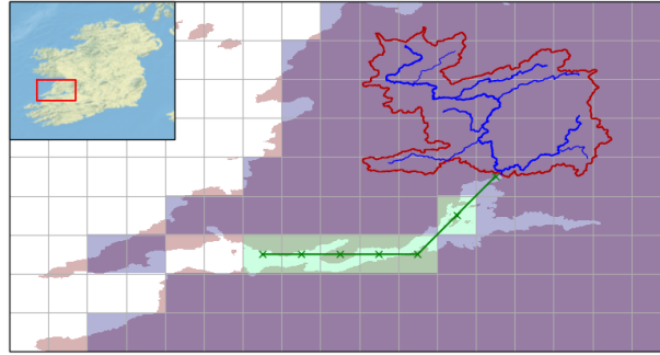
Figure 1. Example of estuary opening: red mask is the HR land mask, blue mask the 12D land mask, green mask represent the 12D cells converted from land to ocean to connect the river basin delineated in red to the ocean.
