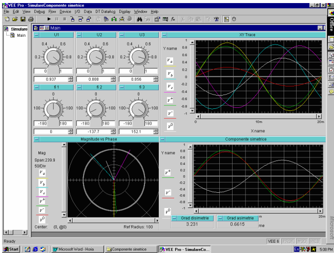
Fig. 2. The simulator interface for direct components.
