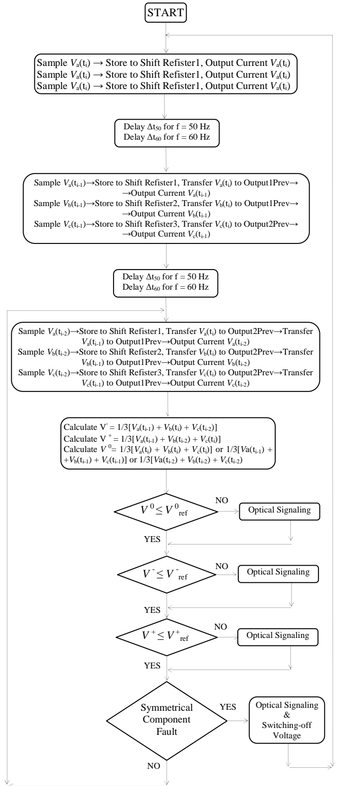
Fig. 3. The flowchart to obtain symmetrical components.
