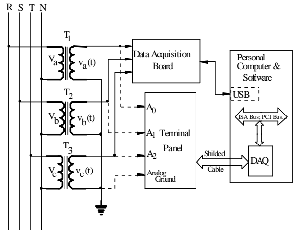
Fig. 8. Basis scheme the virtual instrument.
