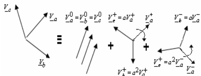
Fig. 1 The symmetrical components of three unbalanced voltages.
