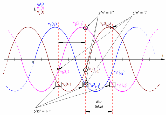
Fig. 4. The voltage samplings and the strategy to obtain symmetrical components.
