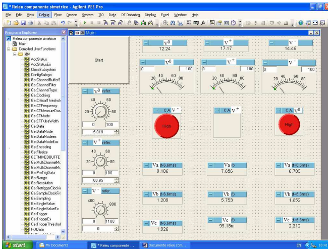
Fig. 7. The graphical relay interface for voltages symmetrical components.
