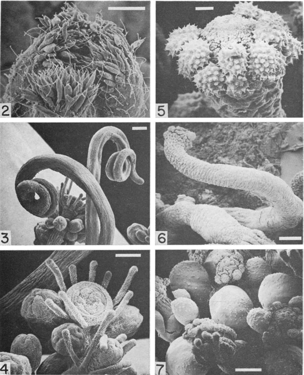
FIGURE 2. Mouth of Podocoryne selena with four lips, each consisting of a battery of about 60 individual pendant microbasic euryteles. Notes the long, flexible, cilia located on the lips and the surface of the manubrium. Scale bar equals 20 \mu\text{m} .
