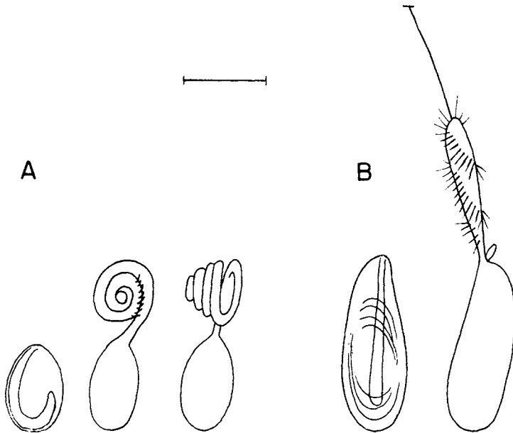
FIGURE 8. Nematocysts of Podocoryne selena and Hydractinia echinata from north Florida, drawn approximately to scale, as seen with phase contrast microscopy. The nematocysts of the two species are not morphologically differentiable. A. Desmonemes. B. Microbasic euryteles. Scale bar equals 5 \mu m.
