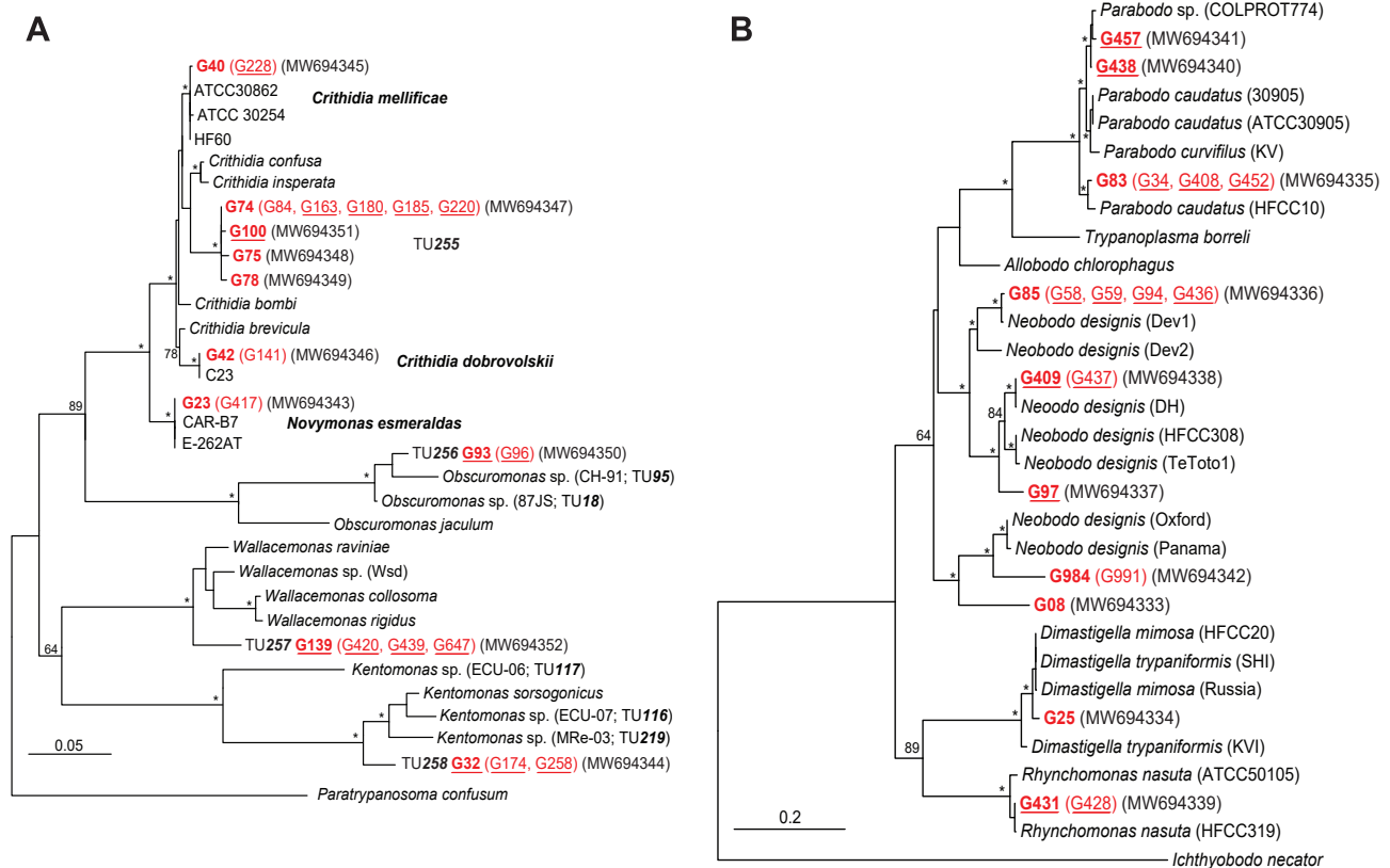
Fig. 1. Phylogenetic trees of monoxenous trypanosomatids (A) and bodonids (B) based on the 18S rRNA gene sequences and reconstructed using the Maximum likelihood method. Asterisks mark branches with maximal statistical support (bootstrap values for maximum likelihood > 90, Bayesian posterior probabilities > 0.95); the scale bar denotes the number of substitutions per site. Newly obtained sequences from tsetse flies (underlined samples are from Glossina (Austenia) tabaniformis (Westwood, 1850), others are from Glossina (Nemorhina) fuscipes fuscipes (Newstead, 1911)) captured in the Dzanga-Sangha Protected Areas, Central African Republic are in red (bold – representative sequences that have been deposited to GenBank, other samples are in parentheses).
