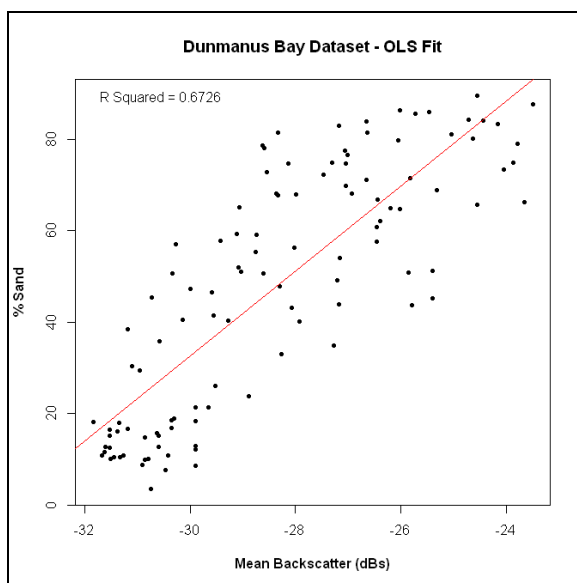
Figure showing the strong linear relationship between Mean Backscatter values averaged over a 20m by 20m grid and the % Sand content of groundtruthing samples collected from Dunmanus Bay, SW Ireland.
