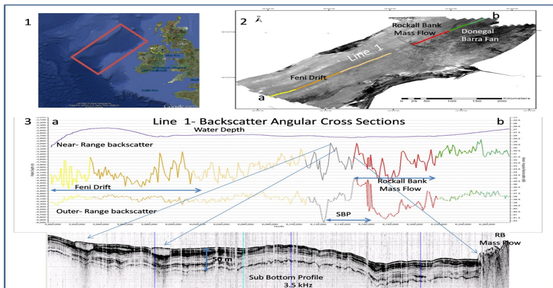
Figure. Panel 1. Index map of the study area. Panel 2. Backscatter mosaic showing position of line 1. Panel 3. Line 1 backscatter cross sections, including near-range and outer-range angular plots. Color intervals in the backscatter plots reflecting sub bottom echo facies. Bottom: shallow seismic record correlated showing change around the Rockall Bank Mass Flow region.
