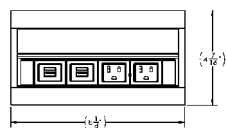
Power Module Standard Configuration
