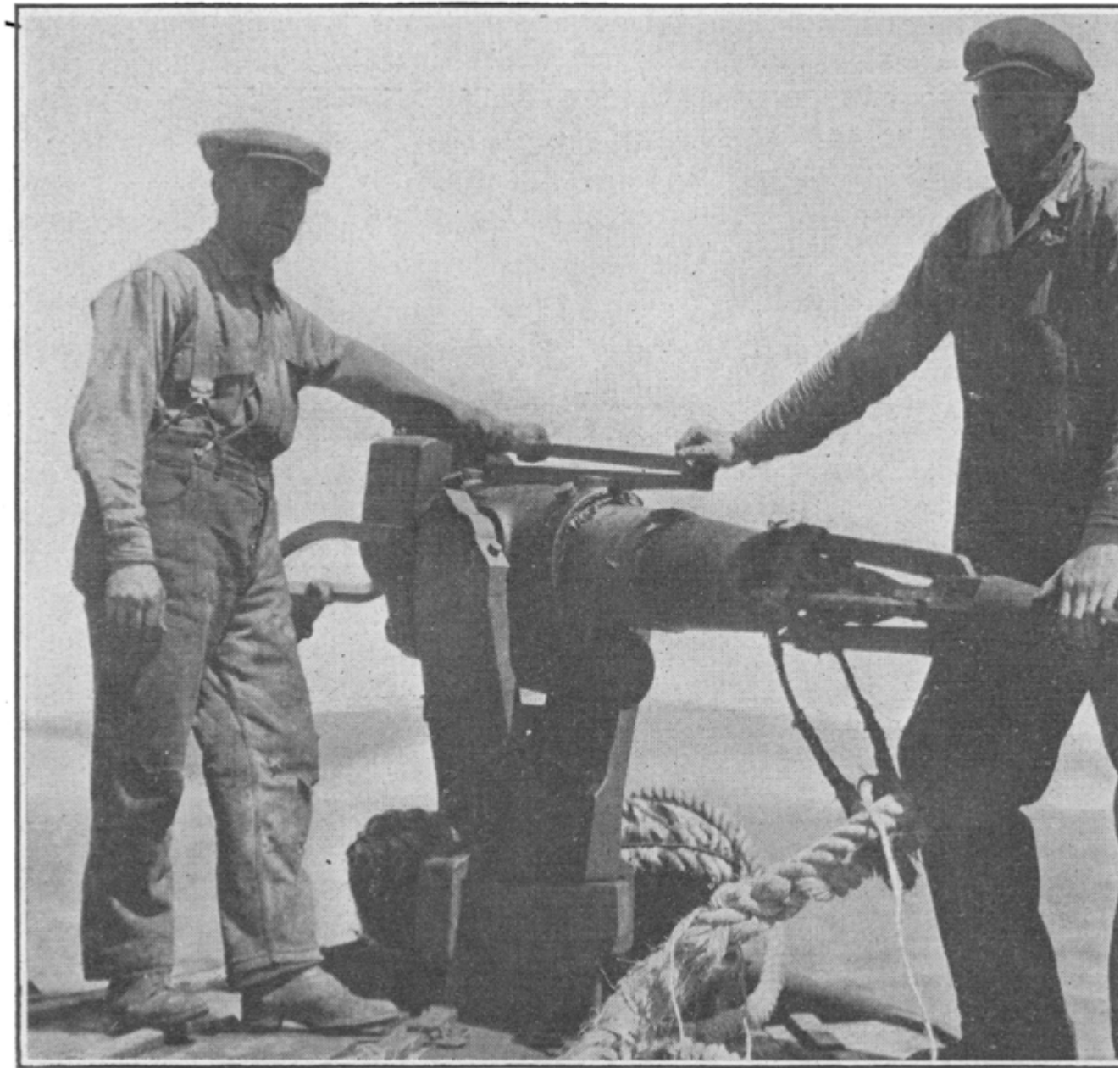
FIG. 1. Whale gun with harpoon loaded. Photograph by O. H. St
