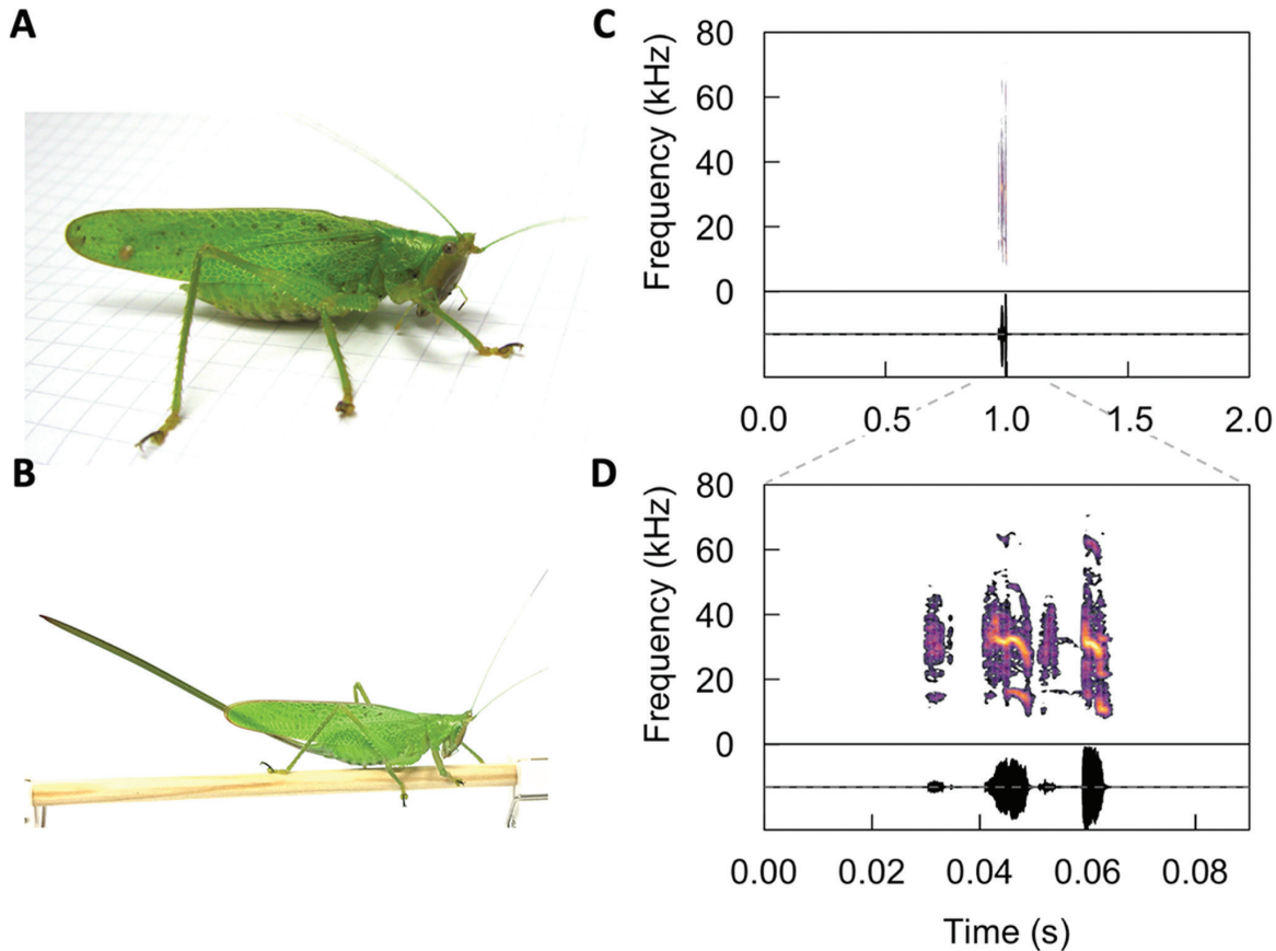
Fig. 5. Photographs and calling song spectrograms of Copiphora breviostris . A. Male (photo credit: H. ter Hofstede); B. Female (photo credit: C. Wilson); C. and D. Spectrogram (top panel) and oscillogram (bottom panel) of one call at different time scales.
