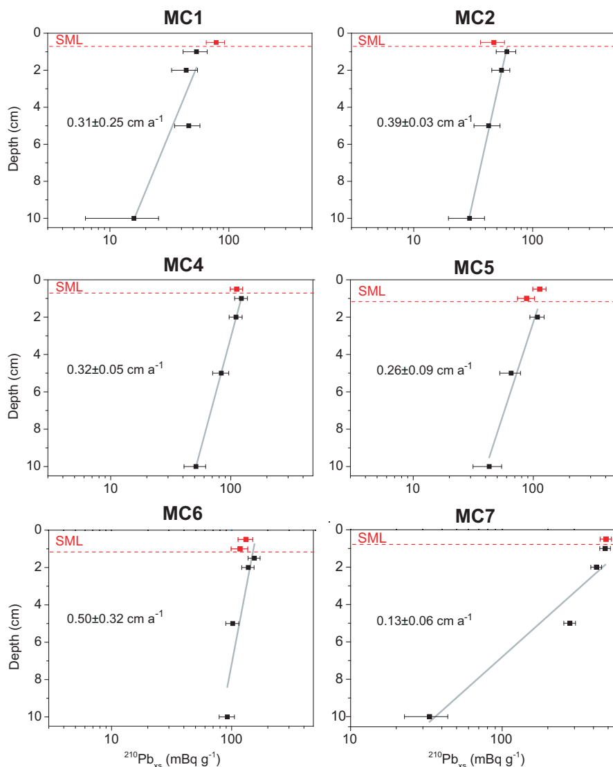
Fig. 2. ^{210}\text{Pb}_{\text{xs}} incorporation into sediment from the sediment surface down to 10-cm depth and the corresponding sediment accumulation rates expressed as \text{cm a}^{-1} . The dashed lines correspond to the limit of the surface mixed layer (SML), also identified as the TAZ. In red are reported the ^{210}\text{Pb}_{\text{xs}} points included in the SML.
