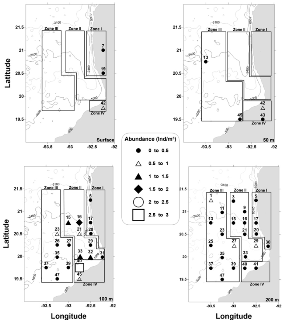
Figure 3. Horizontal distribution of abundances of euphausiids ( \text{Ind m}^{-3} ), adults and early stages at different depths (surface, 50, 100, and 200 m) in the different zones (I, II, III, and IV) of the Campeche Canyon during October of 2012. The geometry of the figures is proportional to the total abundance of euphausiids.
