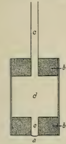
Fig. 1. Apparatus used in testing directly the permeability of the pericarp of Zea : a , membrane; bb , rubber stopper; cc , glass tube; d , receptacle for liquid to be tested.
